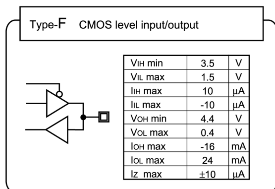
Fig. 2.2 Pin Electrical Characteristics in I/O Circuit Types of MKY35
