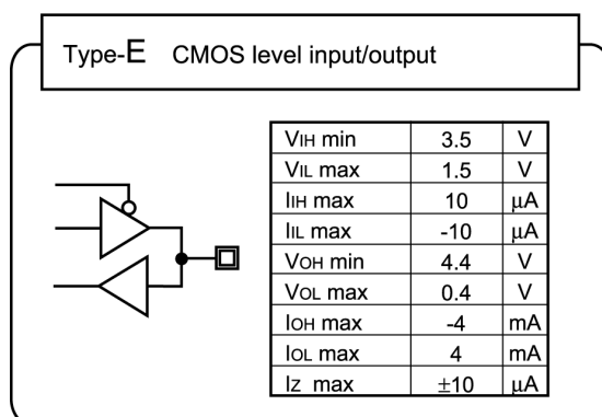
Fig. 2.2 Pin Electrical Characteristics in I/O Circuit Types of MKY35
