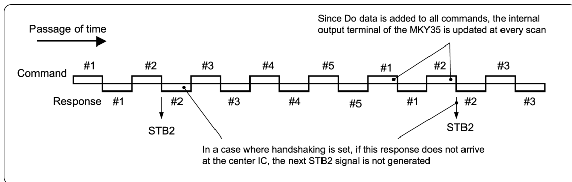
Fig. 4.5 Timing of STB2 Strobe Signal Generation
