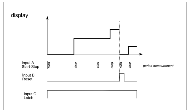
Example 2: cumulated counting with period measurement (start-stop) 4 (F8=1) and activated Latch (Input C)
