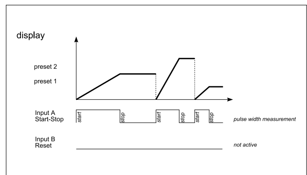
Example 4: defining the time base:
