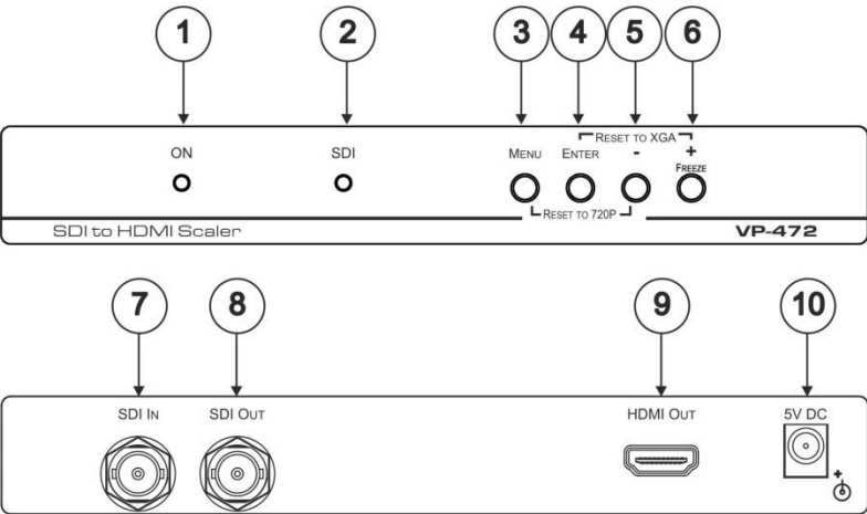
Figure 1: VP-472 SDI to HDMI Scaler
