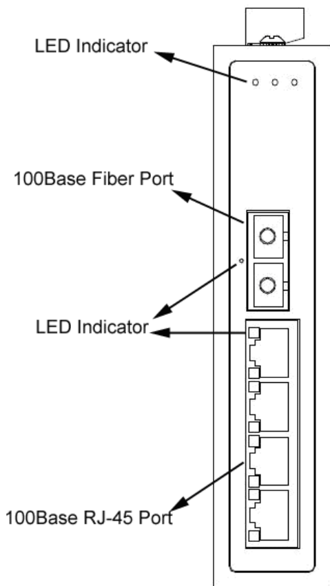
Front Panel of the 4-port 10/100TX + 1 port 100FX Industrial Switch
