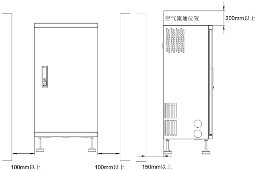
Fig.2-1 Mounting direction and space for V5-JY-4T11G and below power class
