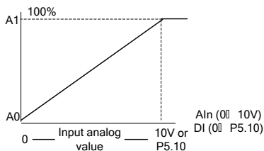
Fig.6-19 Corresponding percentage of input analog value (voltage/frequency)
