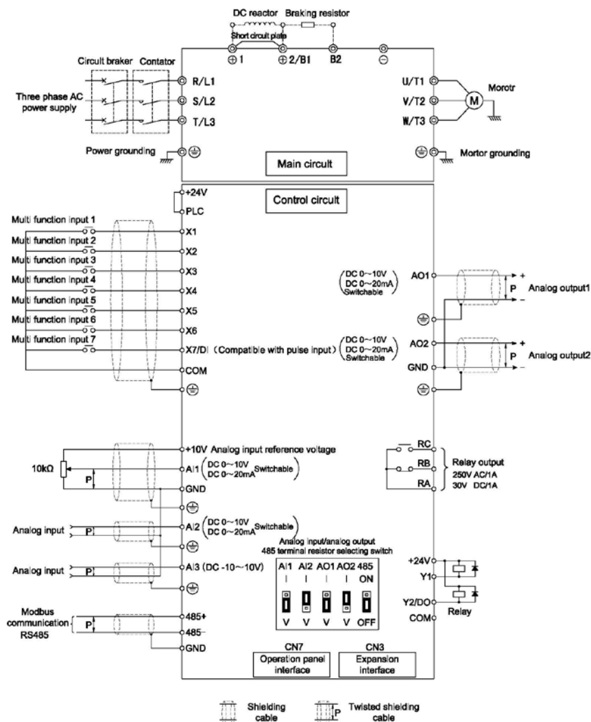
Fig.3-6 Terminal wiring diagram (take V5-JY-4T5.5G/7.5L as an example)
