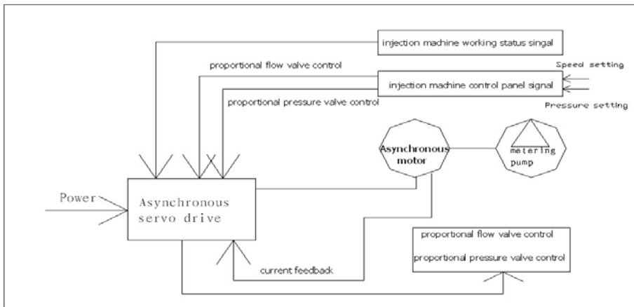
The principle diagram of asynchronous servo drive
