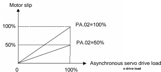
Fig. 6-32 Vector control 1 slip compensation gain
