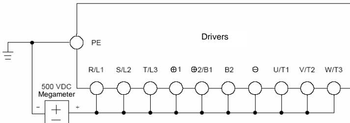
Fig.8-1 Main Circuit Insulation Test for V5-JY-4T11G and V5-JY-4T15G,
