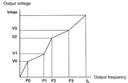
Fig. 6-13 Multi-section V/F curve
