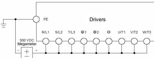
Fig.8-2 Main Circuit Insulation Test for V5-JY-4T18.5G/22L to V5-JY-4T75
