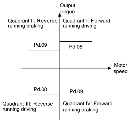
Fig. 6-36 Torque limit
