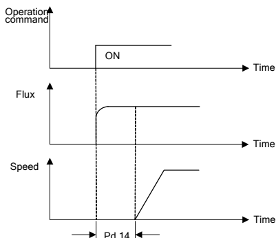
Fig. 6-37 Pre-magnetizing
