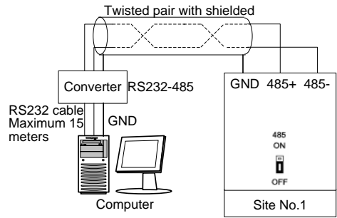
Attached Fig.3 Connecting One asynchronous servo drive to the Computer
