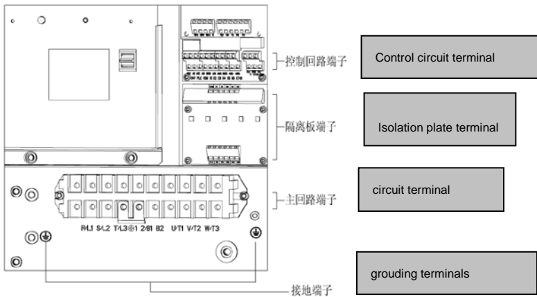
Fig.3-2 Product terminal configuration
