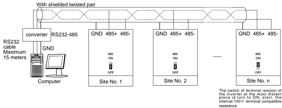
Attached Fig.4 Connecting Multiple asynchronous servo drives to the Computer
