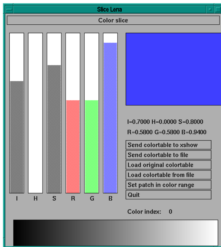
Figure 4.6: Slice window.
