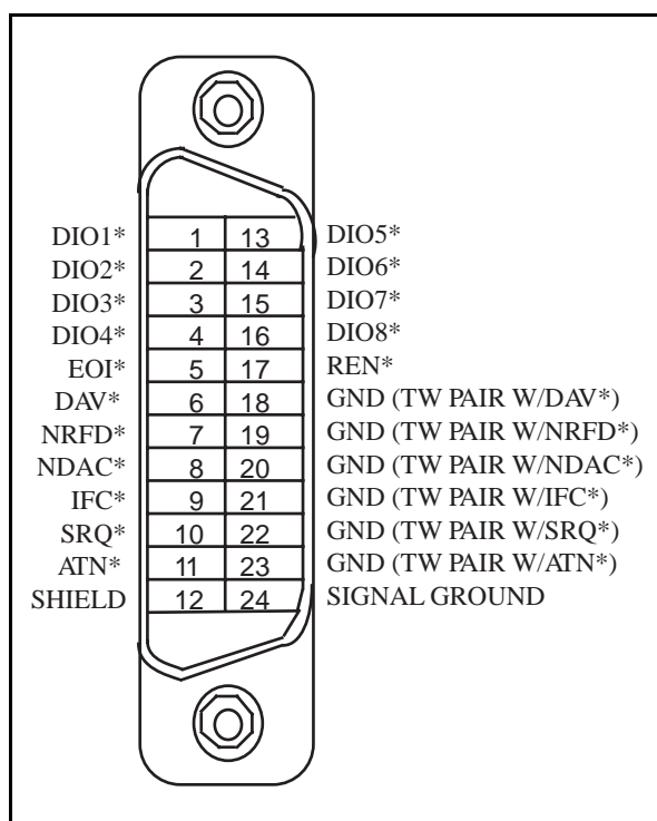
Figure E-1. The GPIB Connector and Signal Assignments
