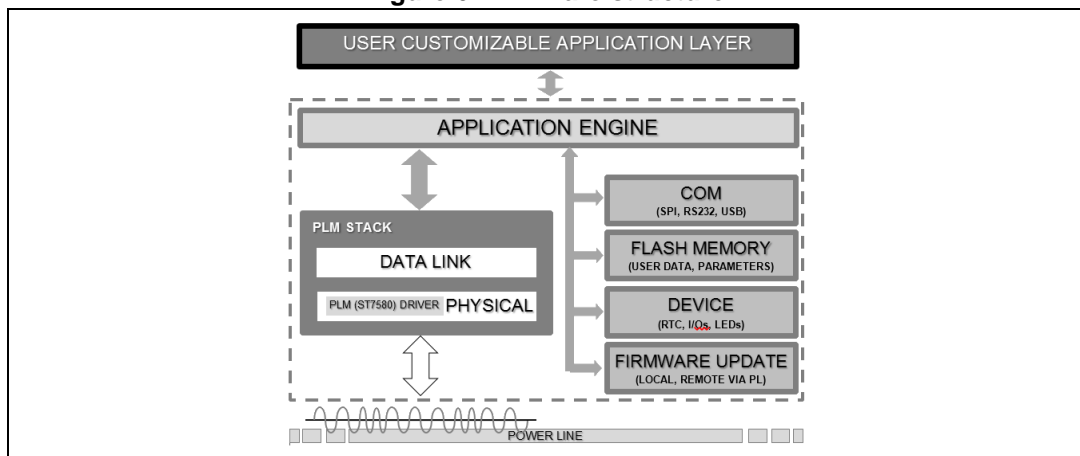
Figure 6. Firmware structure
