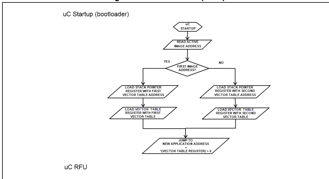
Figure 9. RFU flowchart (2 of 2)
