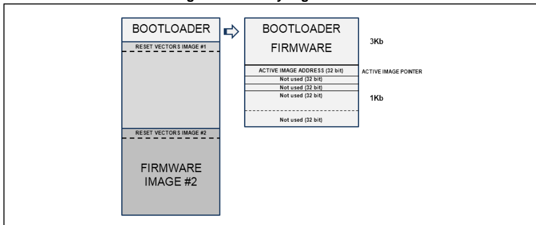
Figure 7. Memory organization
