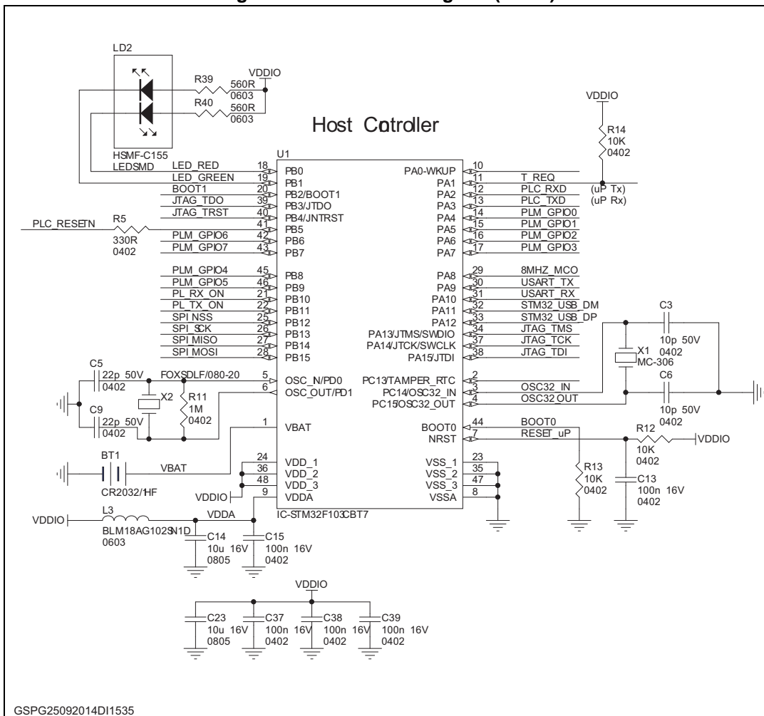
Figure 13. Schematic diagram (2 of 5)
