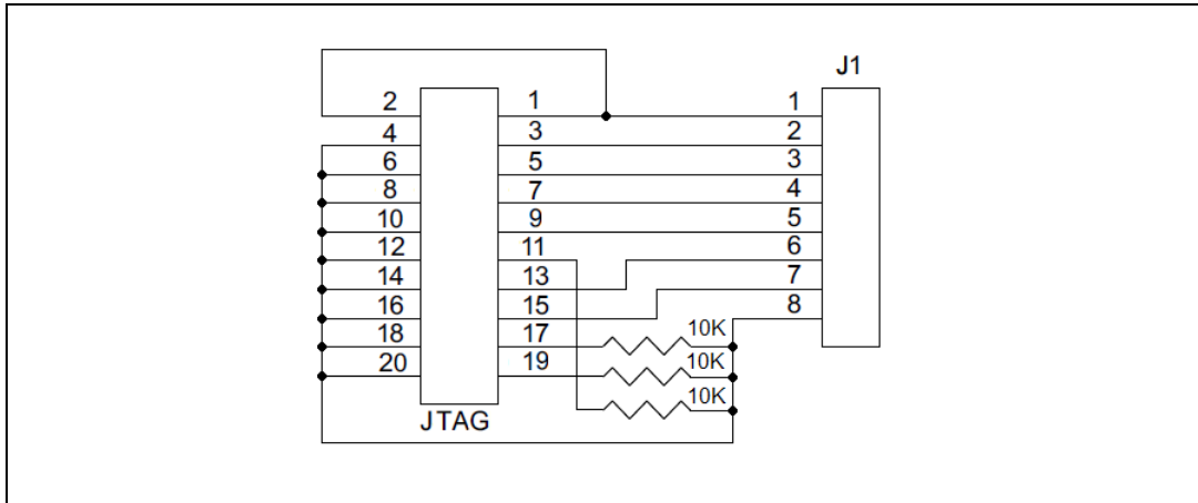
Figure 5. Programming connector JTAG adapter
