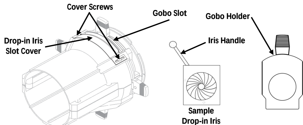
Drop-In Iris/Gobo Slot Location Diagram
