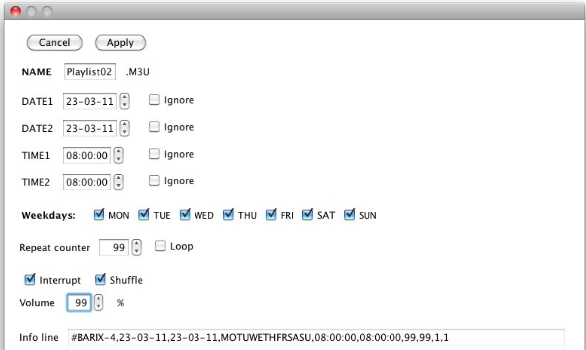
Illustration 3: Playlist manipulation window
