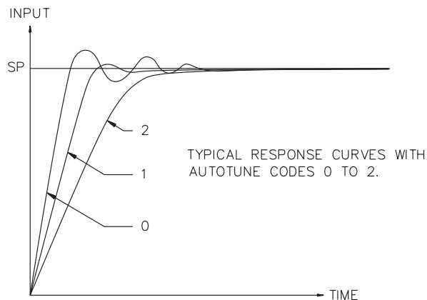
Figure 16, Auto-Tune Code
