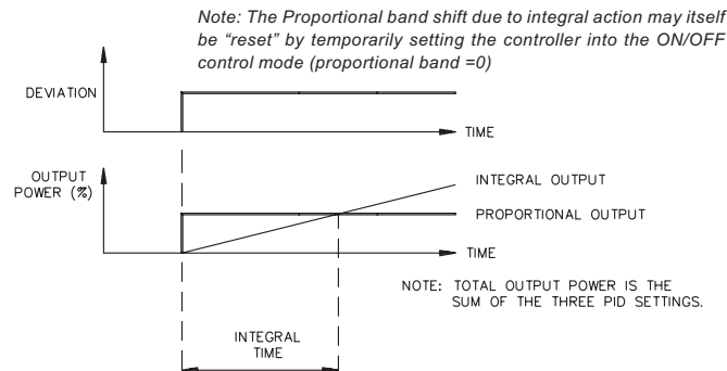
Figure 31, Integral Time
