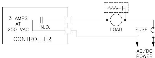
Figure 7, Relay Output
