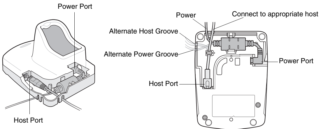
Figure 1-8 Connecting the Cables to the CR0078-P Cradle
