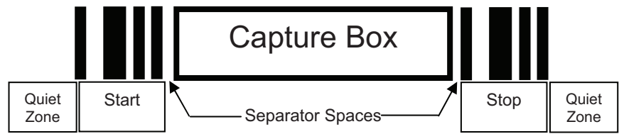
Figure G-2 CapCode Structure
