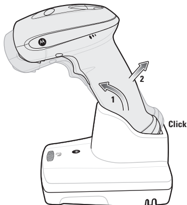
Figure 1-13 Removing the Digital Scanner in the Cradle
