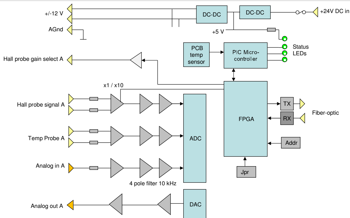
Figure 33. H2O control unit block schematic (channel A shown).
