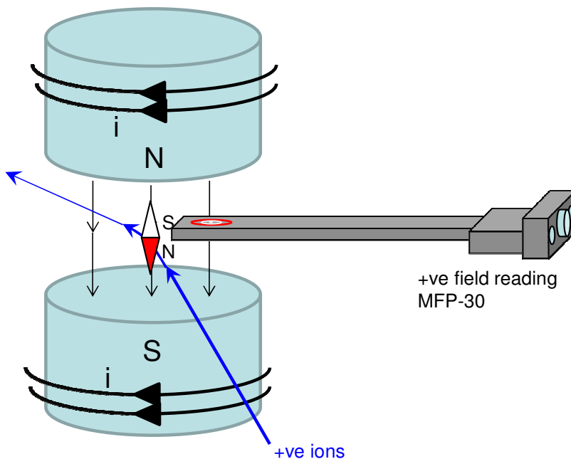
Figure 31. Direction convention for magnetic field lines
