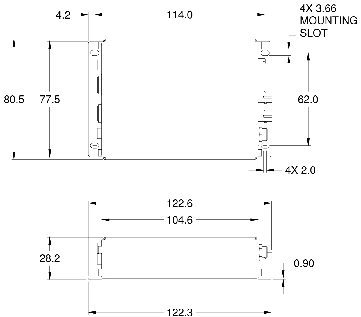
Figure 2. H20 control unit plan and side views. Dimensions mm.
