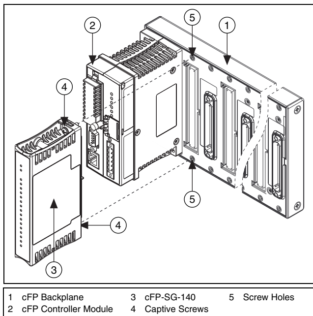
Figure 2. Installing the cFP-SG-140
