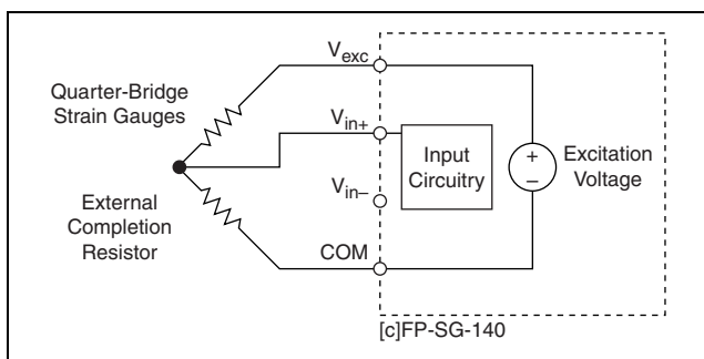
Figure 6. Connecting a Quarter-Bridge Strain Gauge to One Channel
