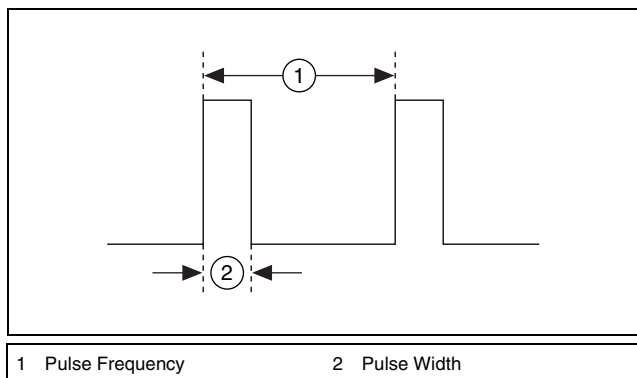
Figure 8. Pulse Width and Pulse Frequency
