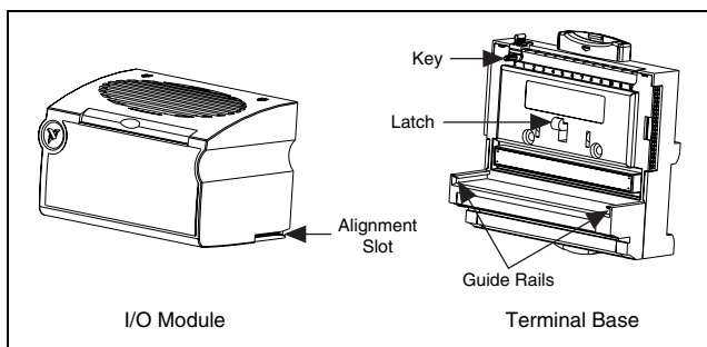
Figure 1. Installing the Module
