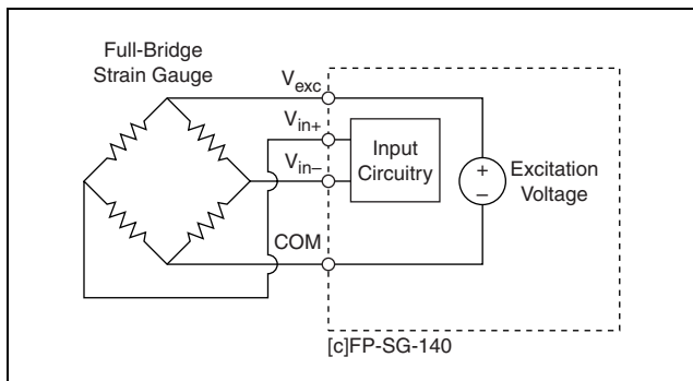
Figure 4. Connecting a Full-Bridge Strain Gauge to One Channel
