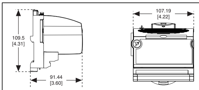
Figure 9. FP-SG-140 Mechanical Dimensions
