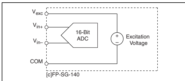
Figure 3. [c]FP-SG-140 Input Circuit
