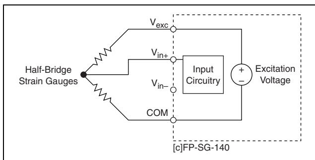
Figure 5. Connecting a Half-Bridge Strain Gauge to One Channel
