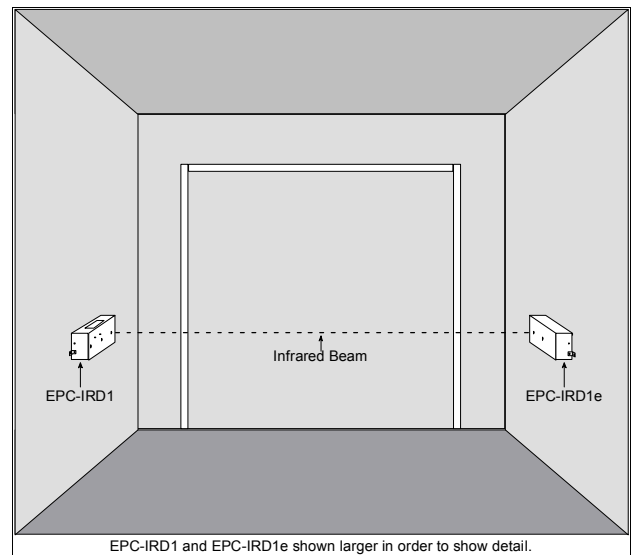
Figure 10b: Example of “front-firing” mounting.
