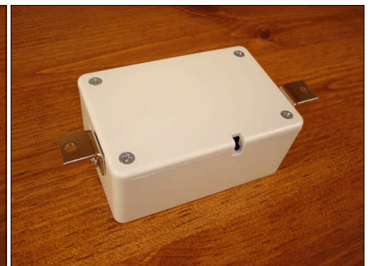
Figure 25b: The rear of the EPC-IRD1 shown with lid secured and front-firing brackets installed.
