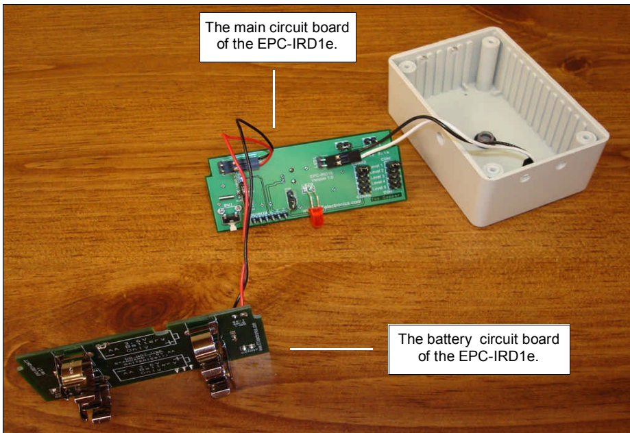
Figure 12: Both circuit boards removed from the optional EPC-IRD1e.
