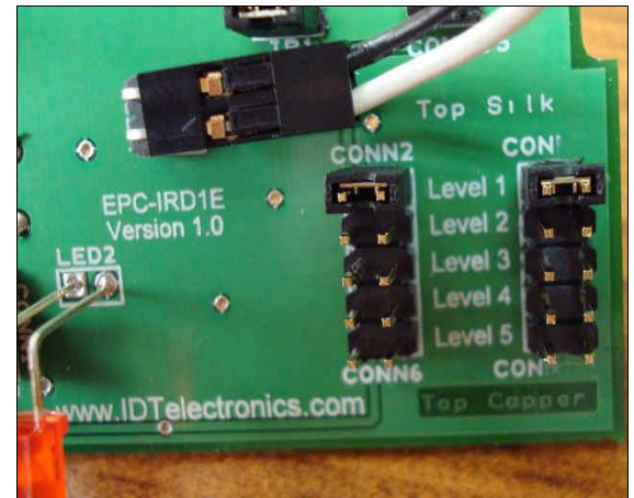
Figure 13: Shown are the five infrared beam level selectors for the EPC-IRD1e. In this photo, you will notice that a jumper is installed on each side of “Level 1.” This means that this EPC-IRD1e
