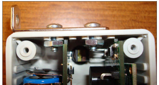
Figure 18b: EPC-IRD1 with "side-firing" brackets installed and both batteries installed. (close-up view)
