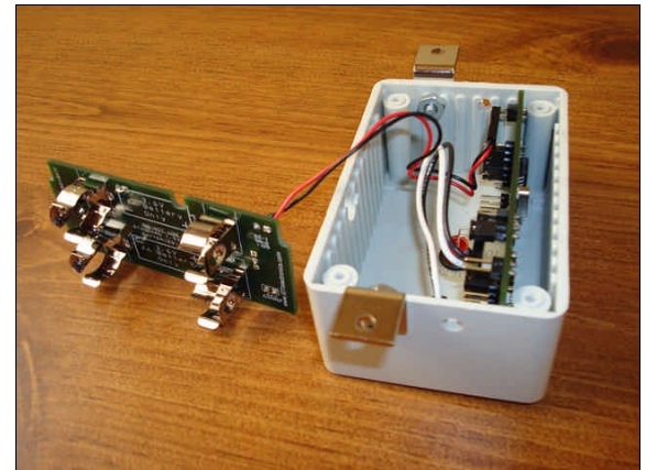
Figure 15b: EPC-IRD1e shown with “front-firing” right-angle brackets mounted to the enclosure.
