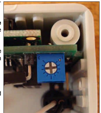
Figure 24: The contrast adjustment screw for the EPC-IRD1 screen.
