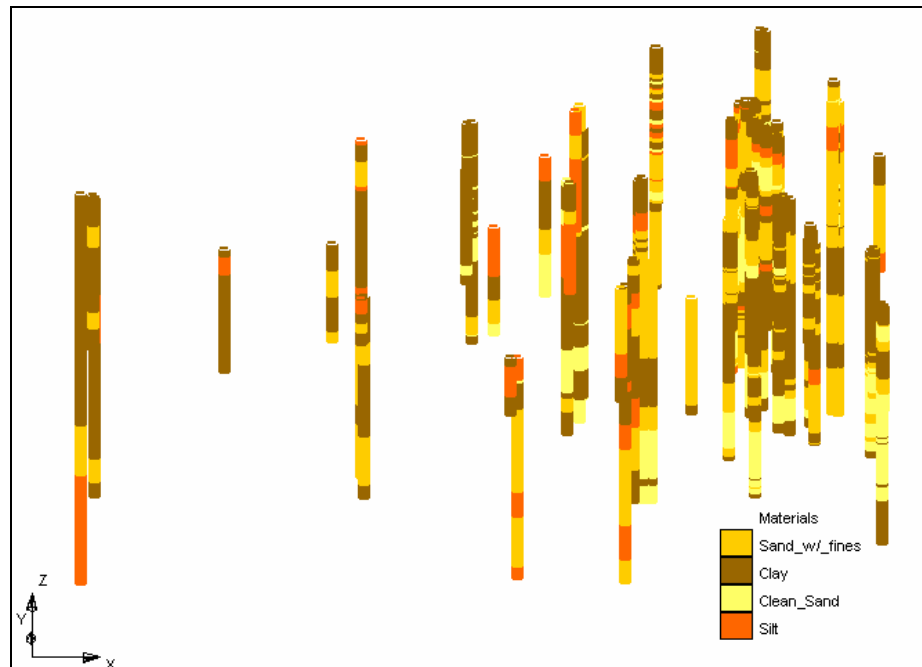
Figure 2.2 3D Oblique View of Borehole Data.
