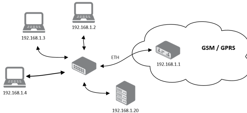
Figure 15: Example 3 Topology of LAN Configuration
