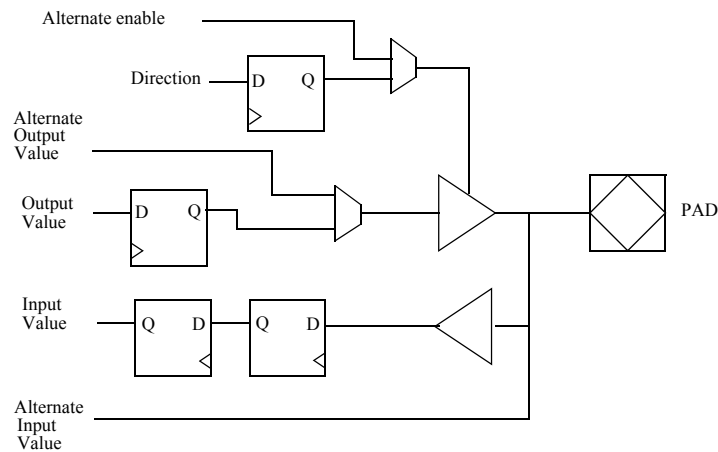
Figure 56. General Purpose I/O Port diagram
