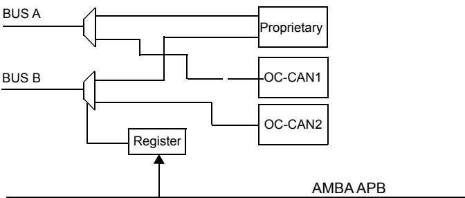
Figure 66. CAN multiplexor
