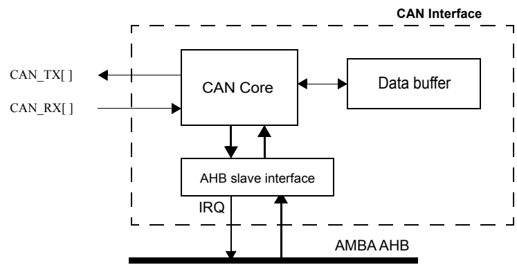
Figure 65. Block diagram
