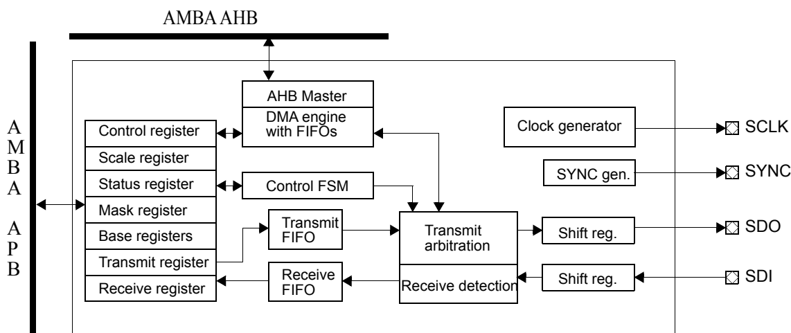
Figure 75. Block diagram
