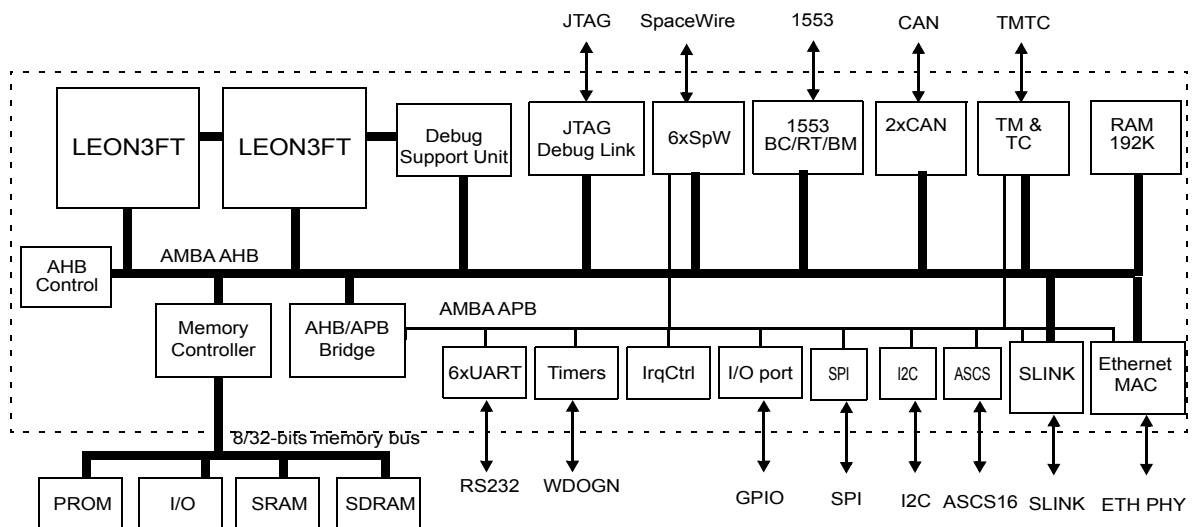
GR712RC Block diagram
