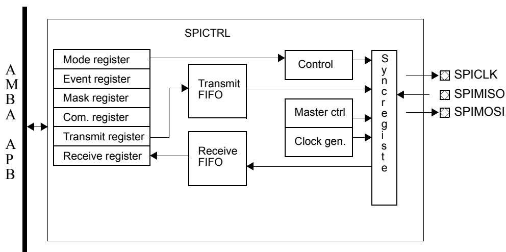
Figure 73. Block diagram
