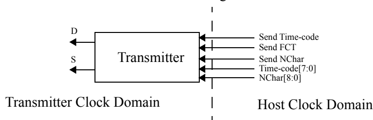
Figure 61. Schematic of the link interface transmitter.
