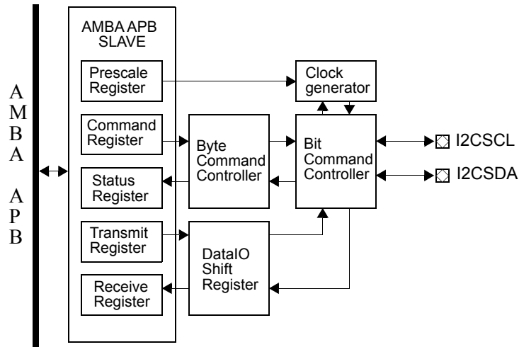
Figure 71. Block diagram
