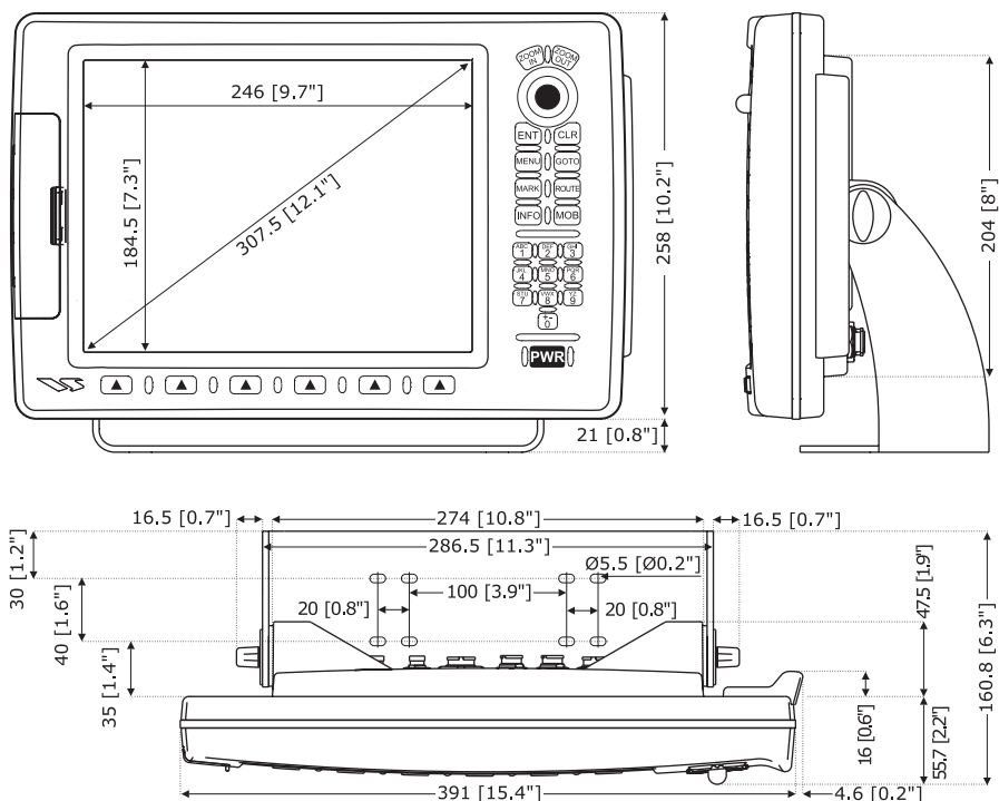
Figure 18.2 - CP500 Dimensions [mm/inch]
