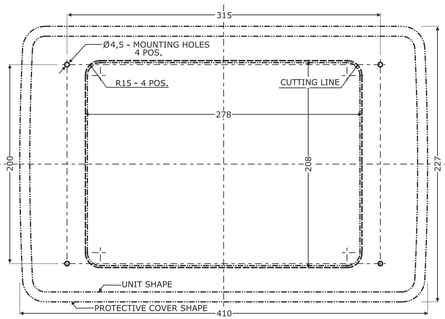
Figure 18.2a - CP500 Flush Mount cutout (Dimensions are in mm)
