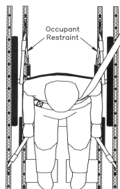
Vertical Floor Track
