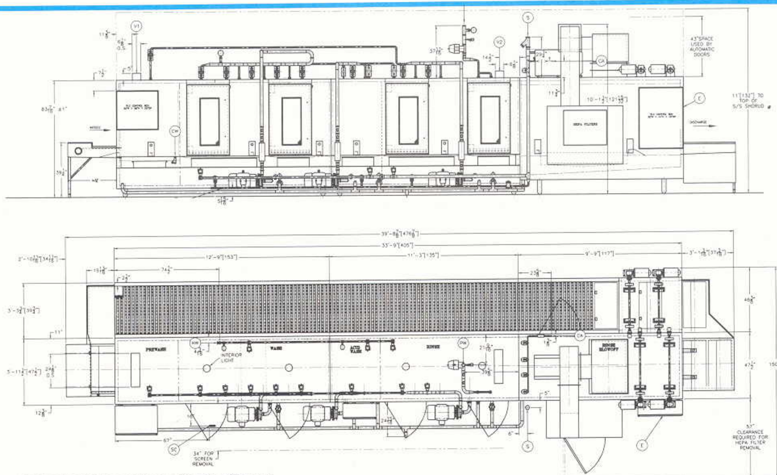
Indexing Glassware Washer/Dryer
