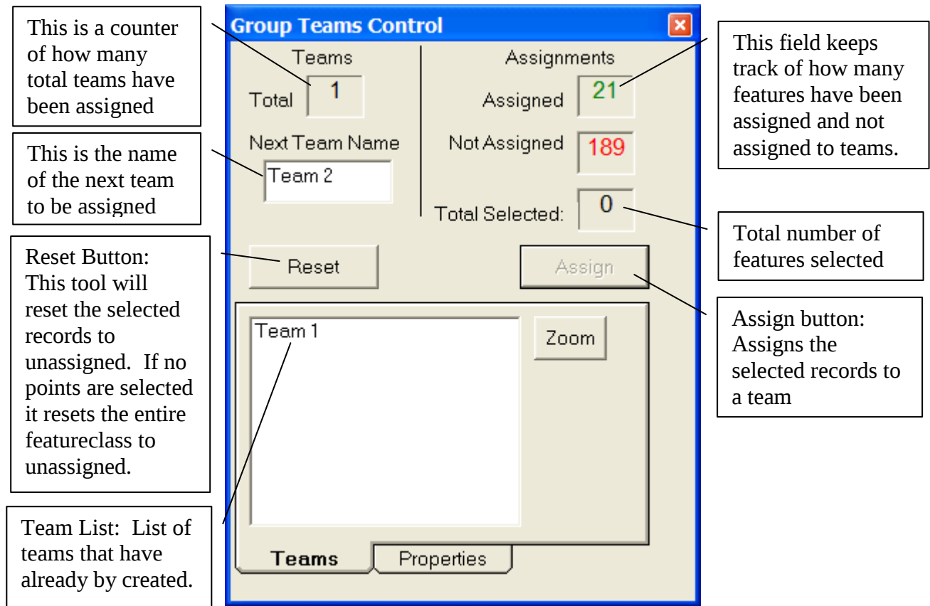
Figure 6. The Group Teams Control is a dockable window that you can place anywhere in your map document. This tool will keep track of your selections and team assignments.
