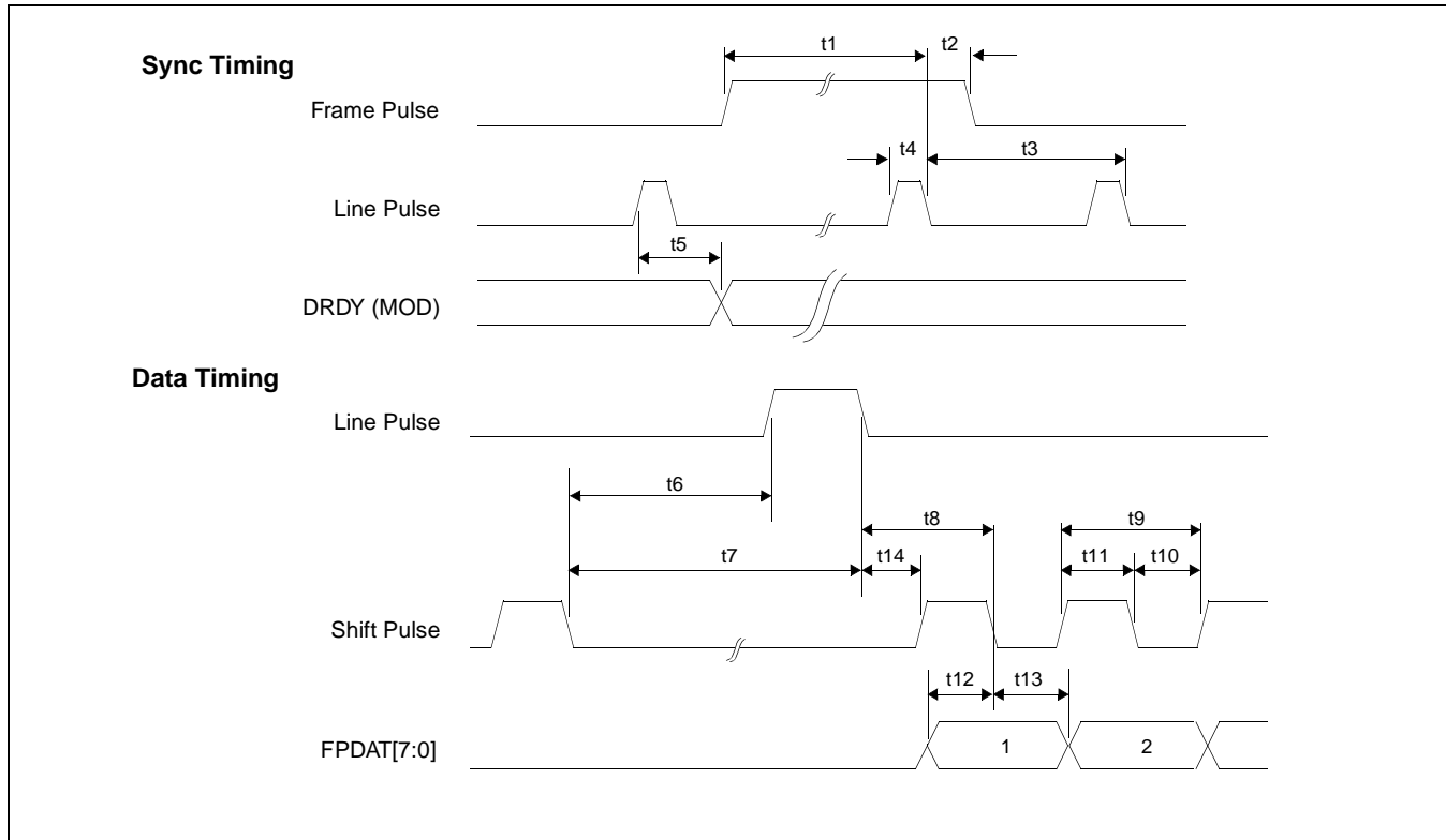
Figure 7-23: Dual Color 8-Bit Panel A.C. Timing
