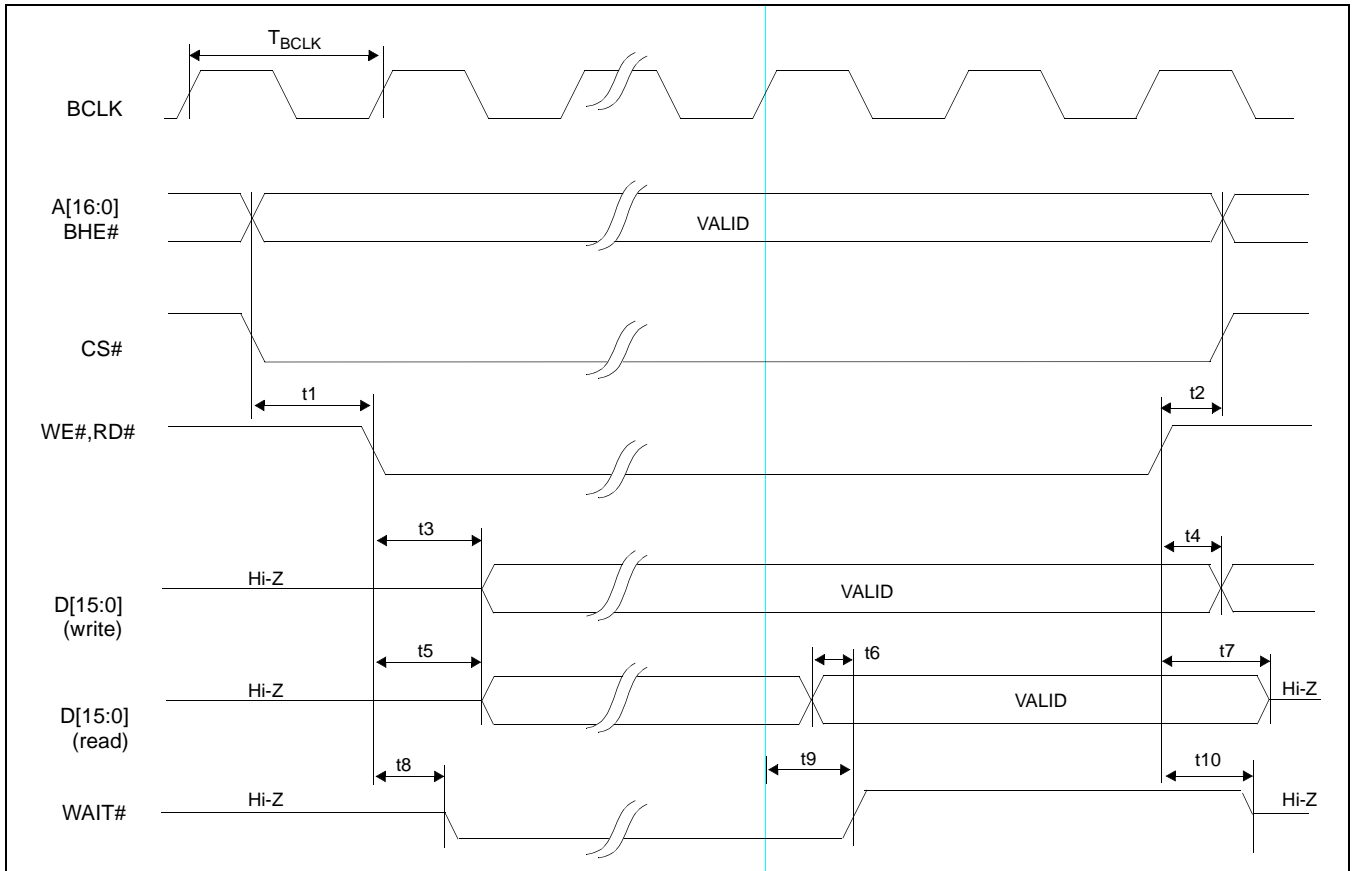
Figure 7-6: Generic #2 Timing
