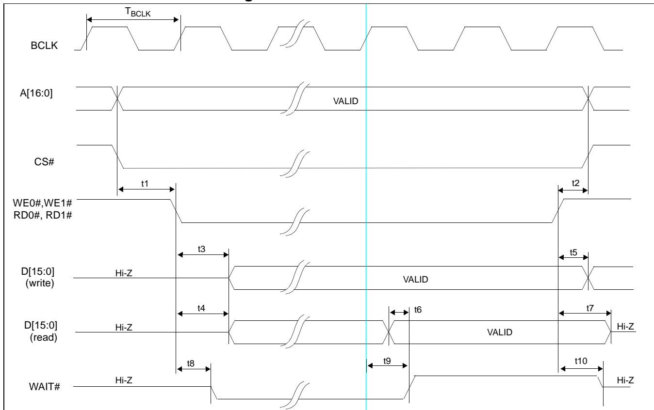
Figure 7-5: Generic #1 Timing
