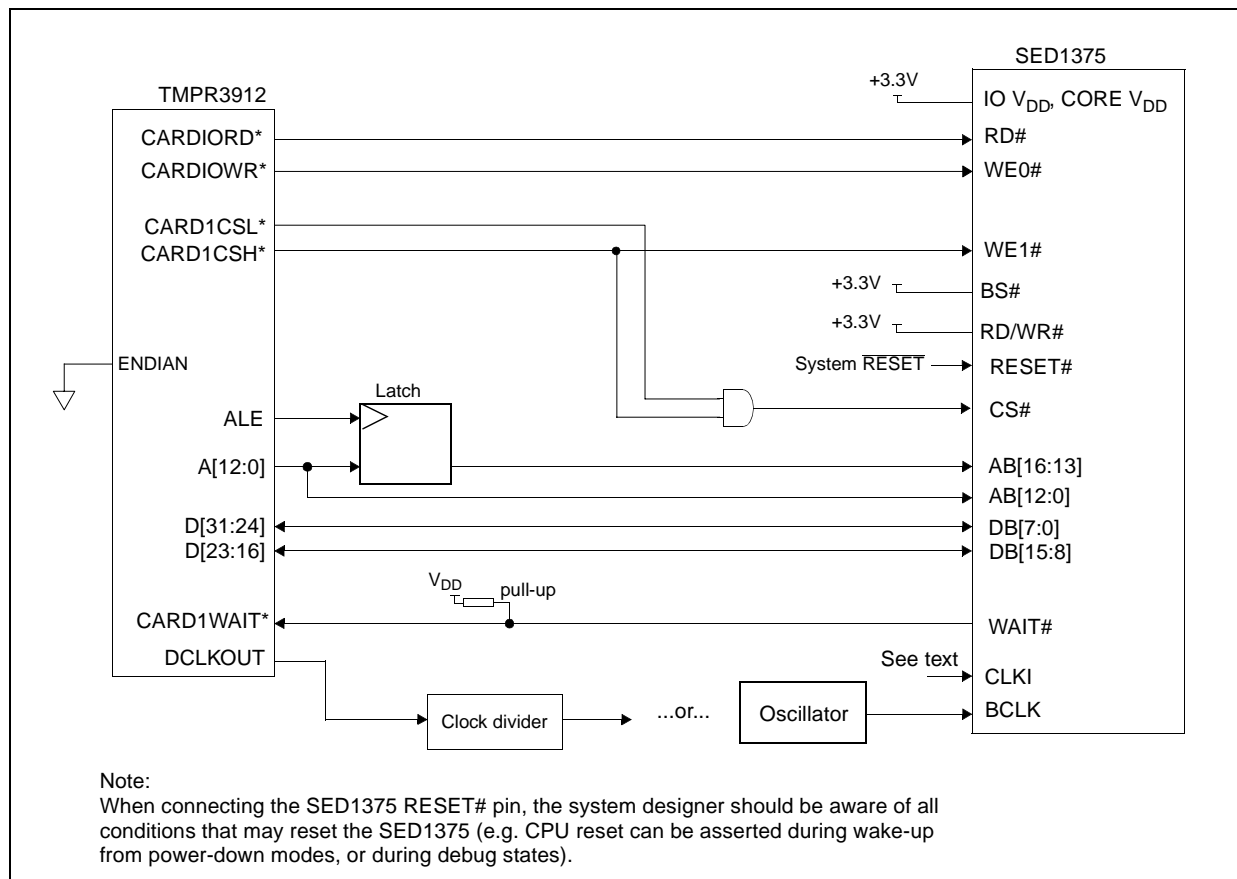
Figure 4-1: SED1375 to TMPR3912 Direct Connection
