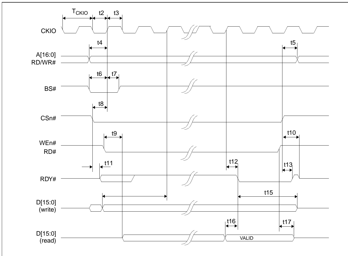
Figure 7-1: SH-4 Timing
