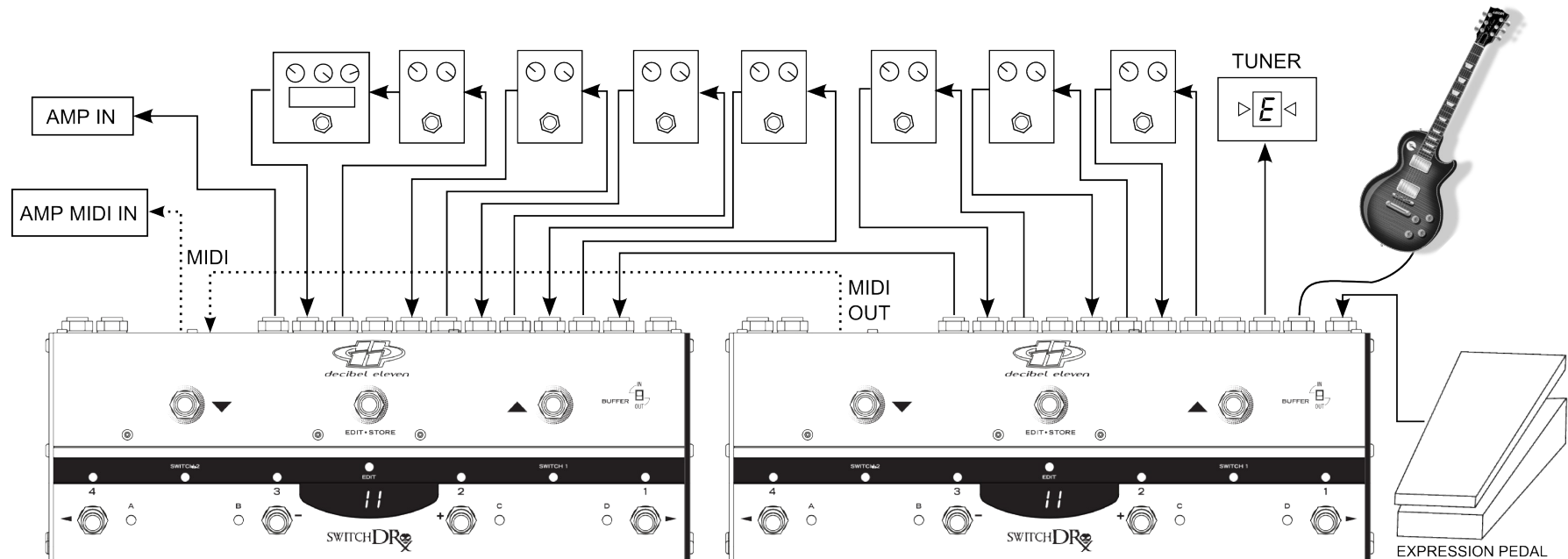
Fig.3 - Expanded setup using two Switch Doctors.
