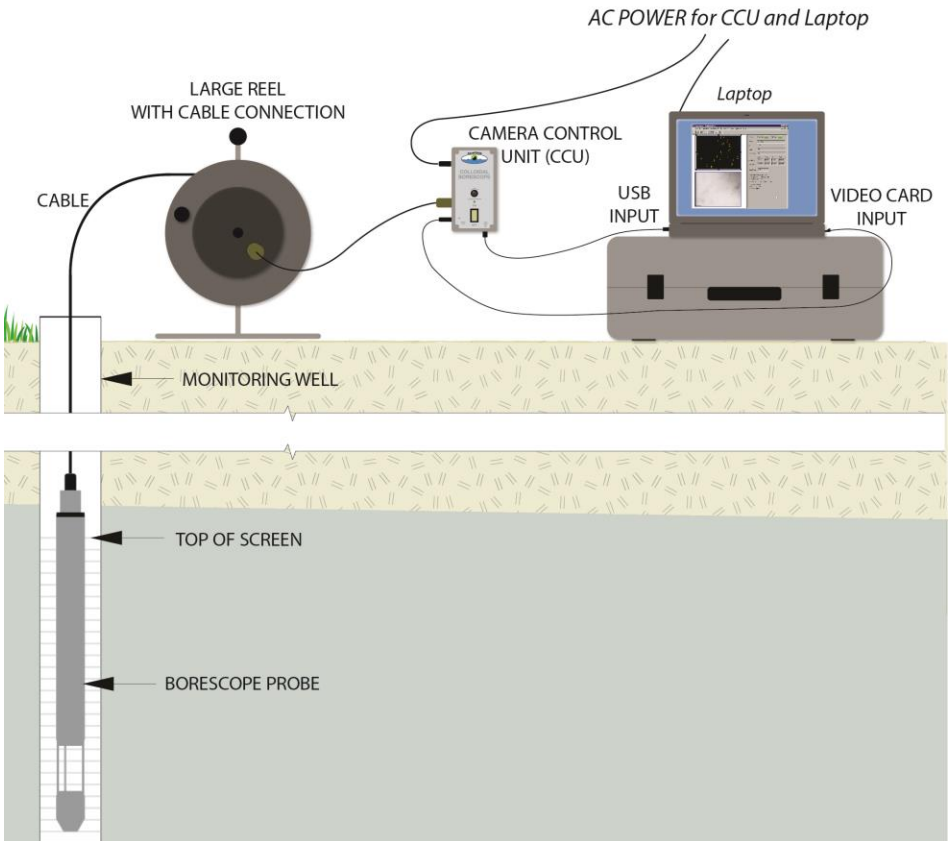
Figure 1.2 –Colloidal Borescope System Schematic
