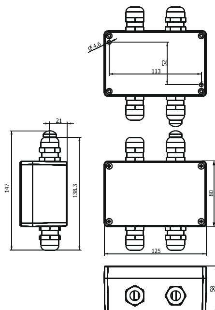
Junction box
