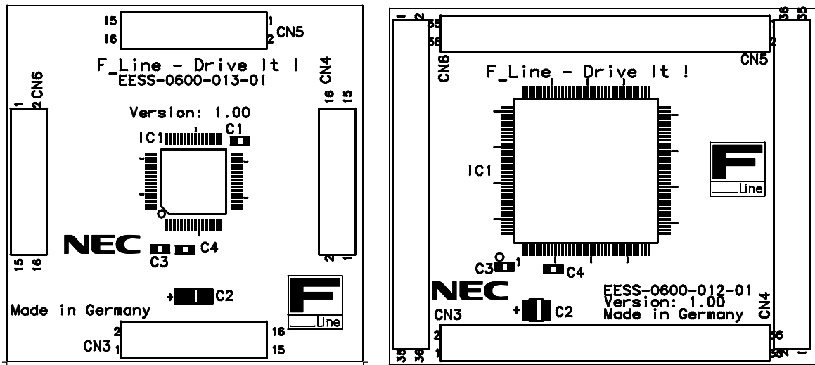
Figure 3: F_Line - Drive it! CPU module components
