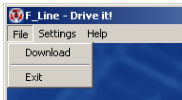
Figure 9: File menu
