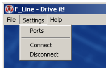
Figure 6: Settings menu
