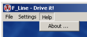
Figure 11: Help menu
