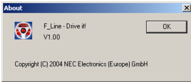
Figure 12: About box
