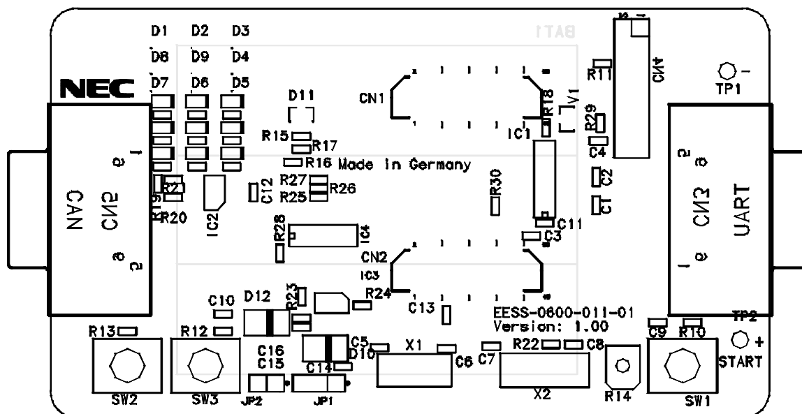
Figure 2: F_Line - Drive it! baseboard jumpers, connectors, switches and LEDs
