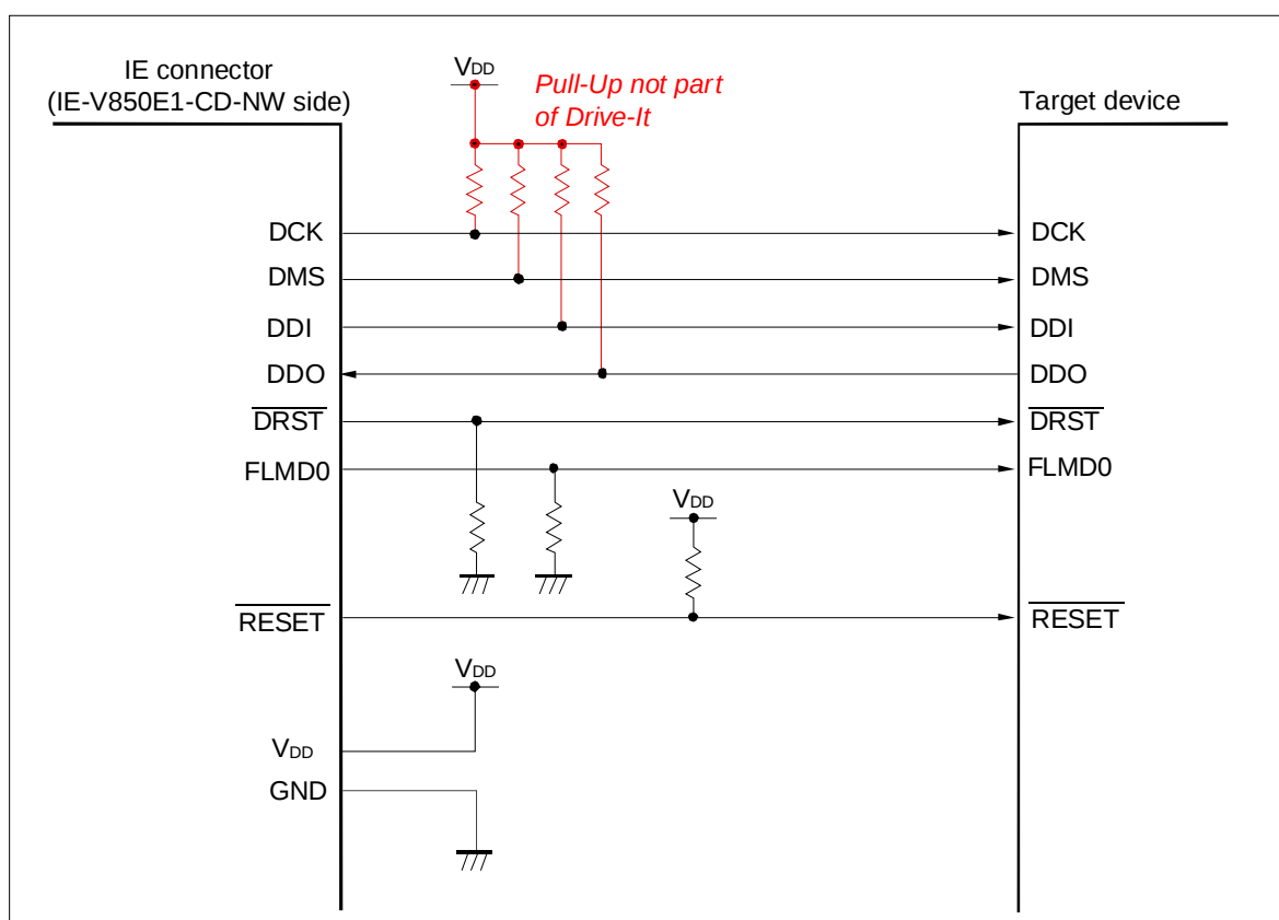
Figure 4: N-Wire Connection Circuit Example
