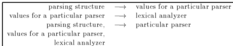
Figure 1: Module Dependencies
