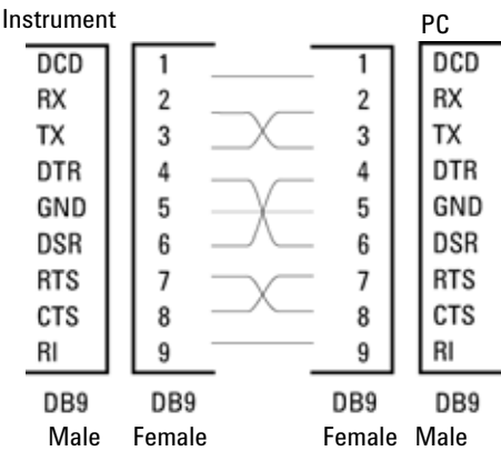
Figure 56 RS-232 Cable
