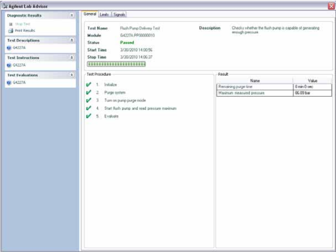
Figure 36 Flush pump delivery test – Test Passed
