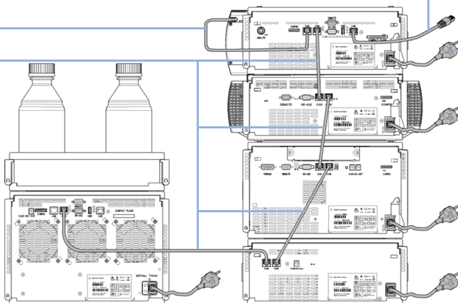
Figure 16 Supported Two Stack Configuration Rear View (Standard)
