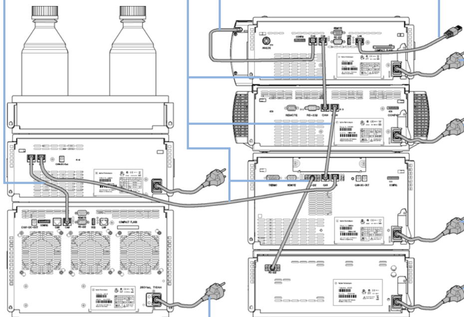
Figure 18 Supported Two Stack Configuration Rear View (Thermostatted)
