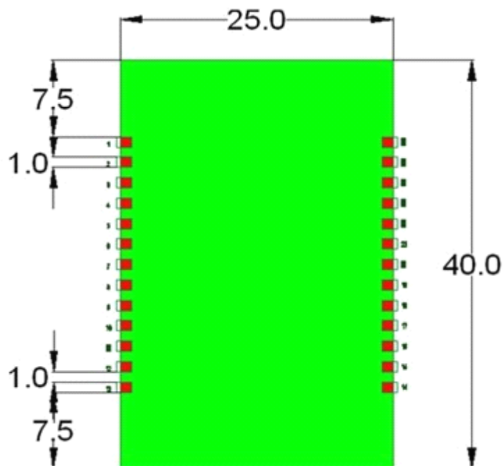
Figure 12 USR-WIFI232-Ca/Cb Mechanical Dimension
