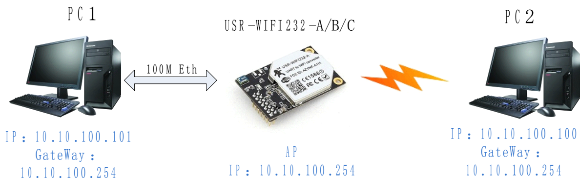
Figure 26 USR-WIFI232-A/B/C Ethernet Interface Networking (As AP)
