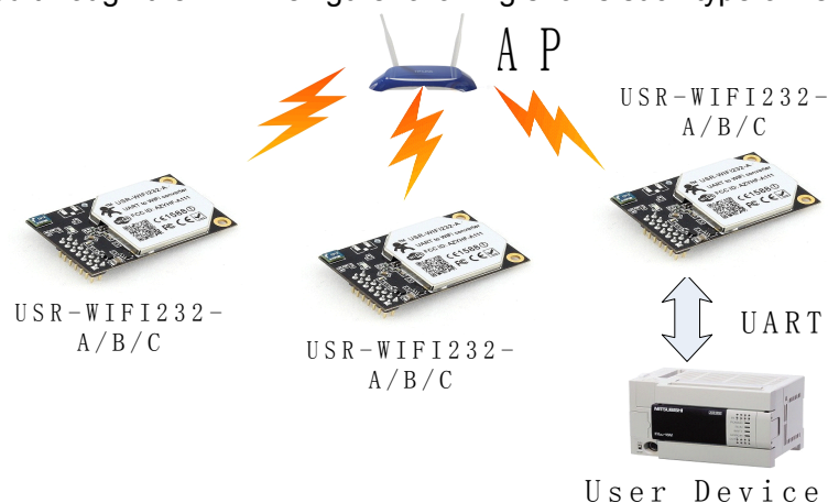
Figure 23 USR-WIFI232-A/B/C Basic Wireless Network Structure
