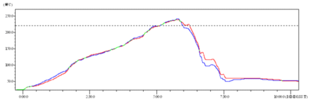
Figure 5 Reflow Soldering Profile
