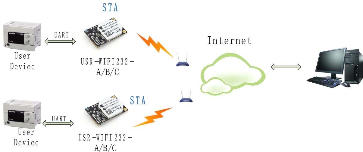
Figure 55 Remote Management Application
