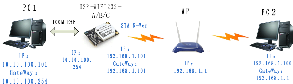
Figure 27 USR-WIFI232-A/B/C Ethernet Interface Networking (As STA, N-Ver)
