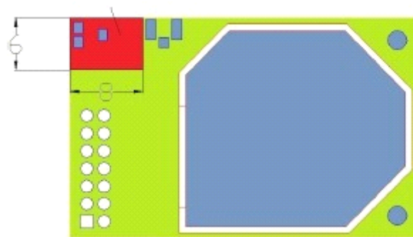
Figure 13 USR-WIFI232-A/B/C Chip Antenna Keep Out Region
