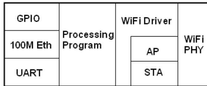
Figure 22 USR-WIFI232-A/B/C Functional Architecture
