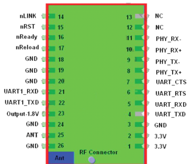
Figure 10 USR-WIFI232-Ca/Cb Pins Map
