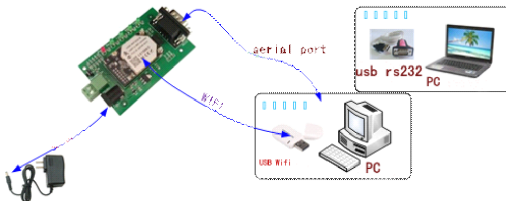
Figure 50 Connection diagram
