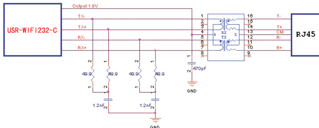
Figure 18 Ethernet Reference Design with Transformer
