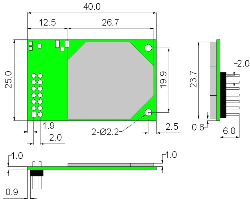
Figure 11 USR-WIFI232-A/B Mechanical Size
