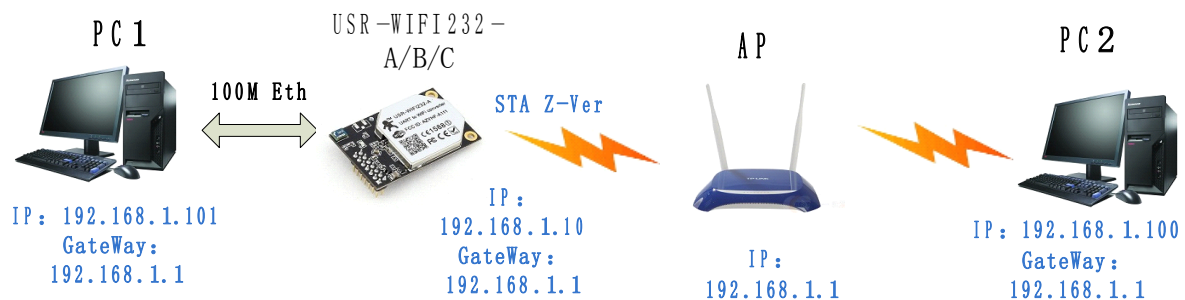
Figure 28 USR-WIFI232-A/B/C Ethernet Interface Networking (As STA, Z-Ver)
