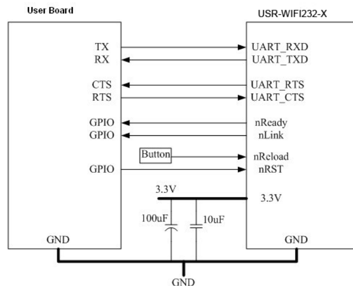
Figure 17 USR-WIFI232-A/B/C Hardware Typical Application
