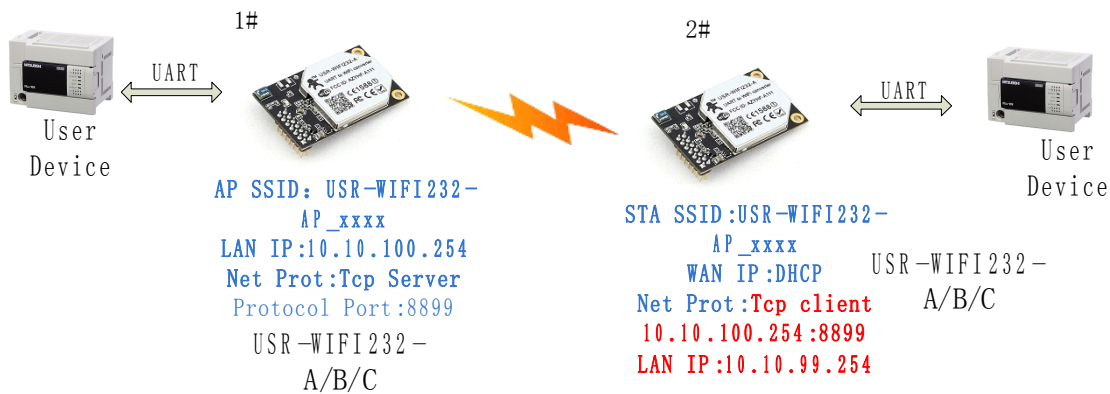
Figure 56 Transparent Serial Port Application
