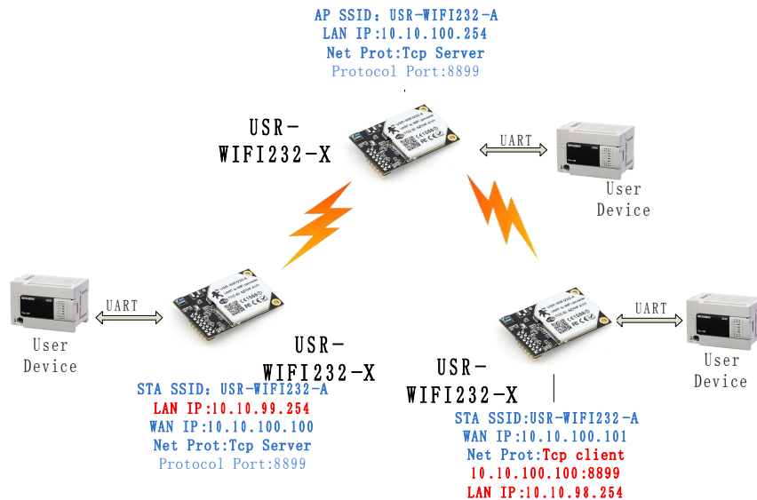
Figure 65 Two USR-WIFI232-A/B/C Modules Connection Through AP
