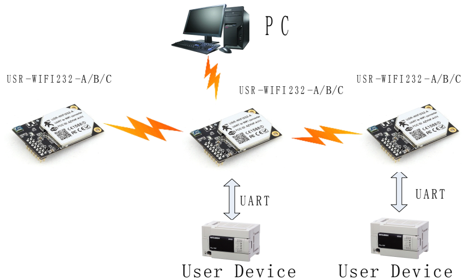
Figure 24 USR-WIFI232-A/B/C STA Network Structure
