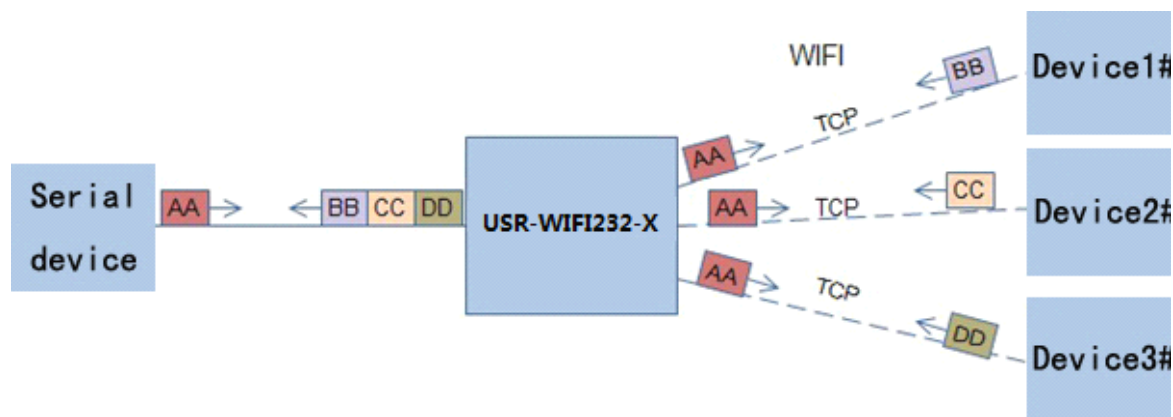
Figure 30 Multi-TCP Link Data Transmission Structure
