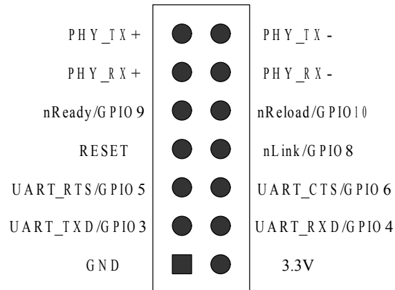
Figure 8 USR-WIFI232-A/B Pins Map
