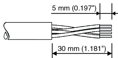
Figure 2-14 Preparing the cable
