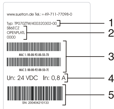
Figure 2-17 Nameplate (example)
