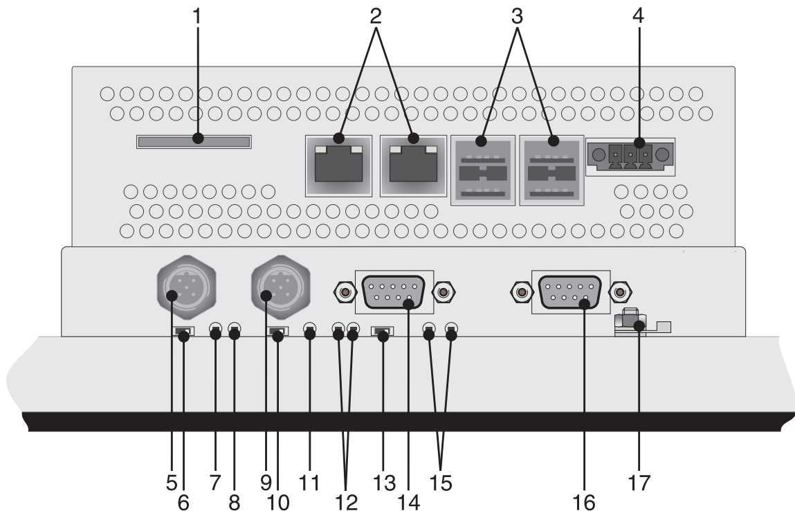
Figure 4-7 Rear view CAN
