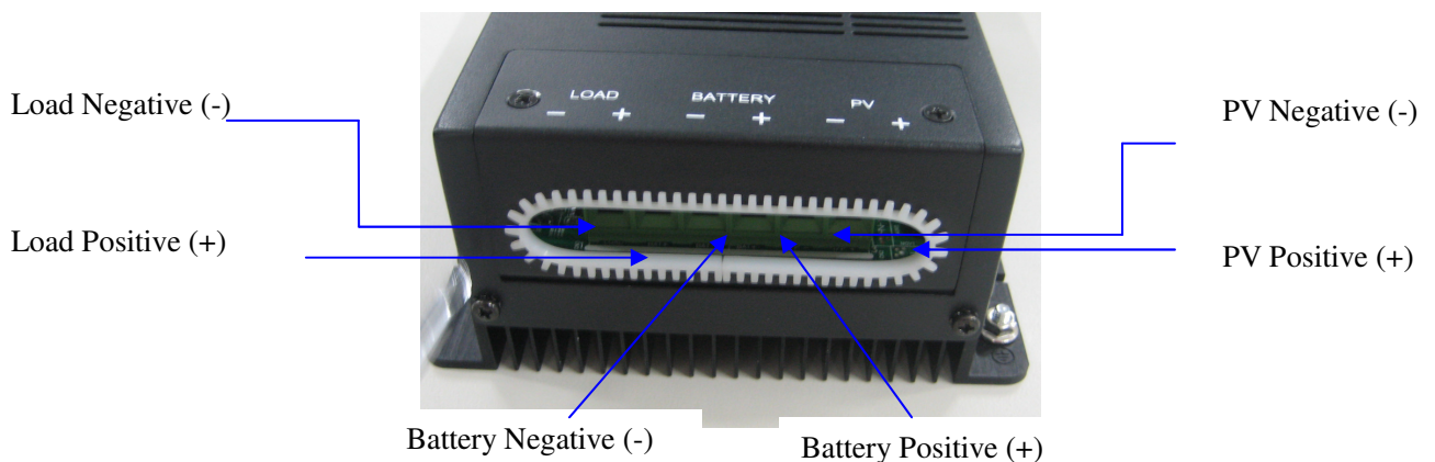
Figure 1 – 9: PV charge control mode wiring
