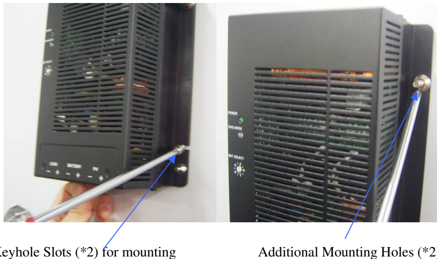
Figure 1 – 5: Mounting the Solar charge controller
