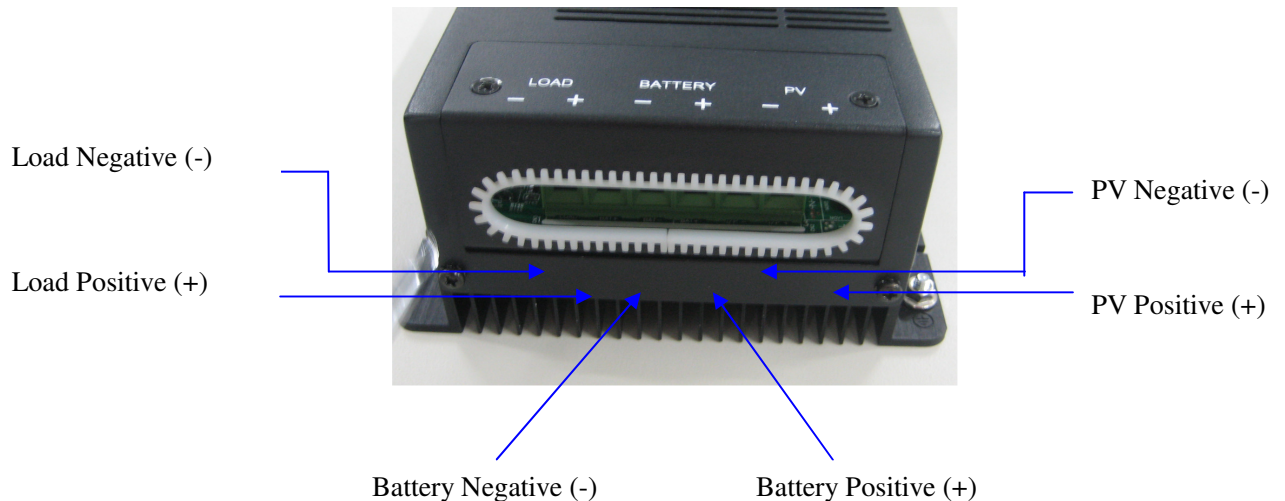
Figure 1 – 8: DC terminal connector location
