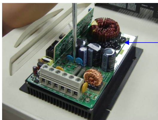
Figure 1 – 7: Safety (Earth) ground
