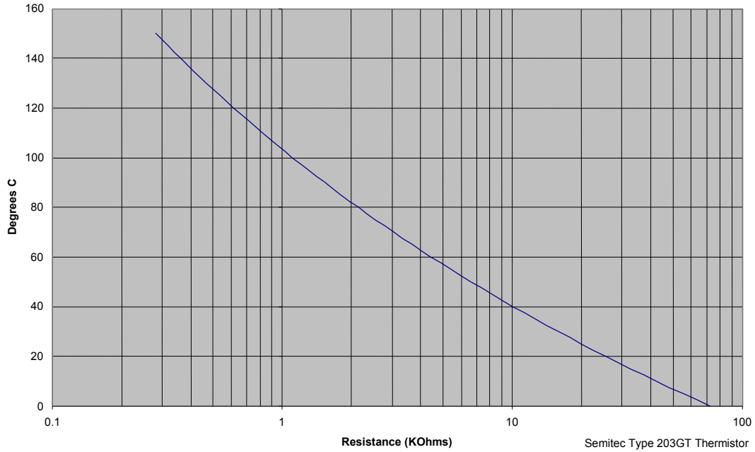
Figure 14. Thermistor Chart
