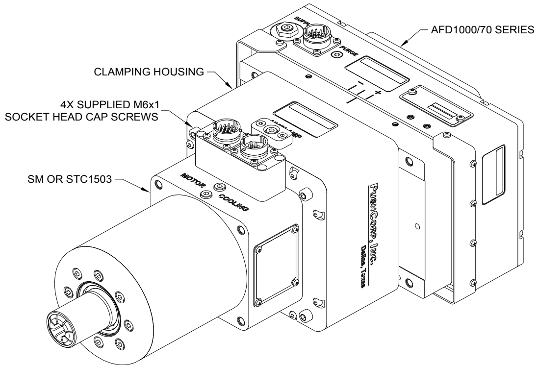
Figure 1. 1503 Parallel-Axis Configuration
