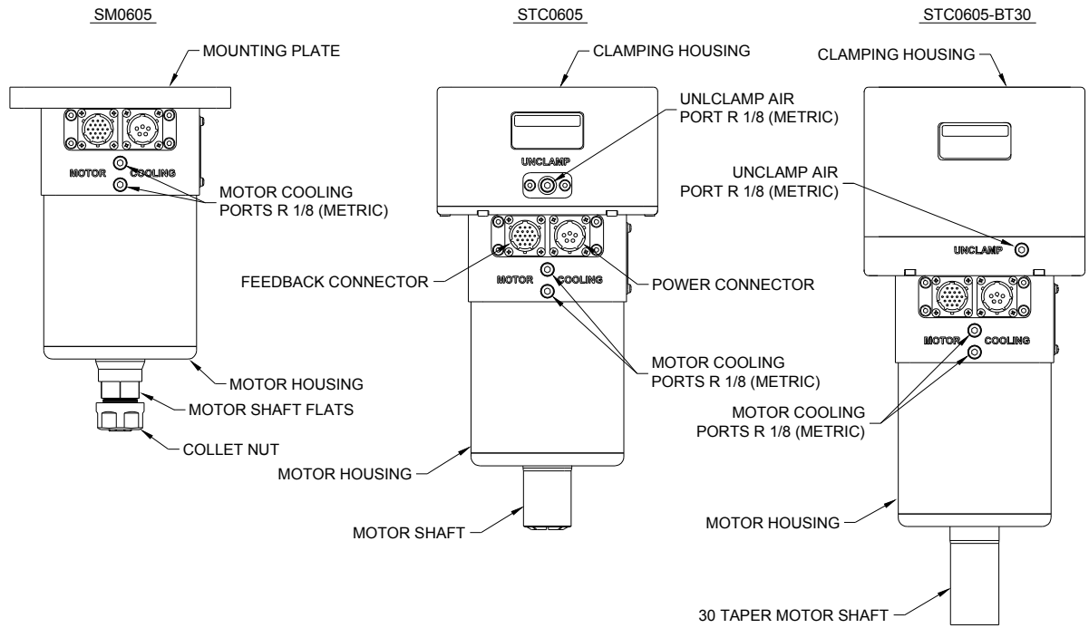
Figure 13. 1503 External Features
