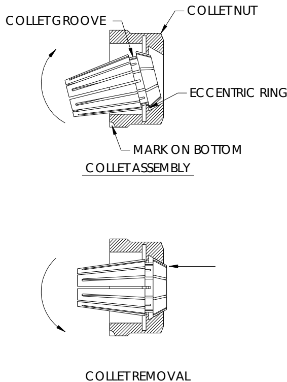
Figure 10. SM Collet Assembly and Removal
