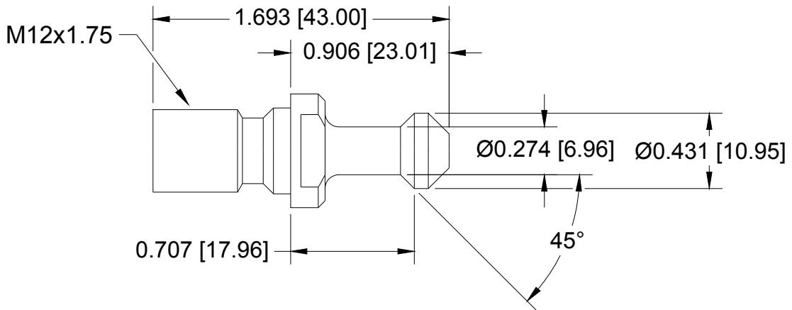
Figure 9. BT30 Retention Knob
