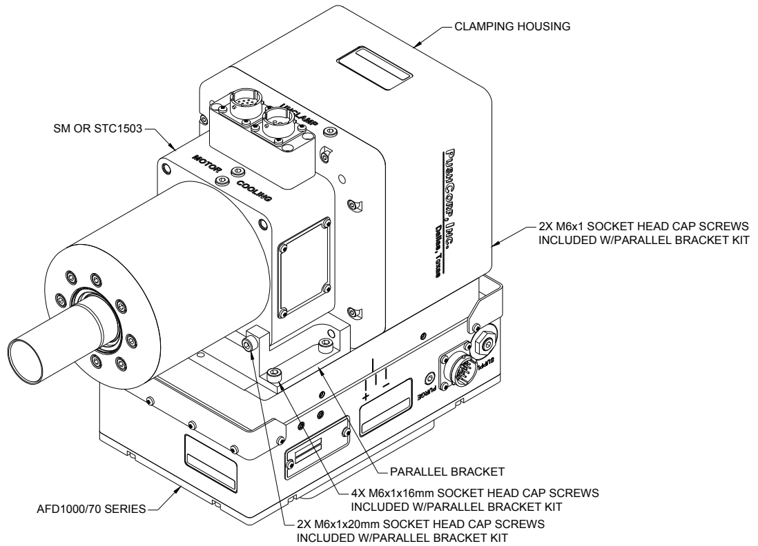
Figure 1. 1503 Parallel-Axis Configuration
