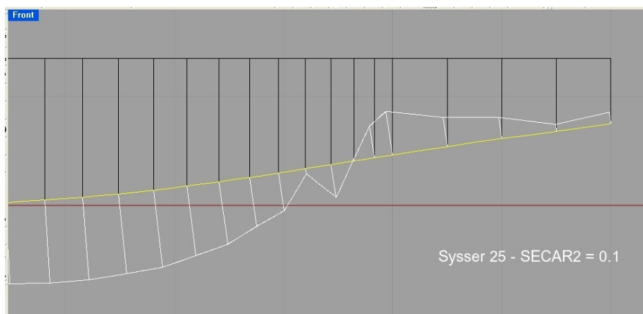
Fig. 4. Stern of the vessel, side view, curvature SECAR 2 = 0.1
