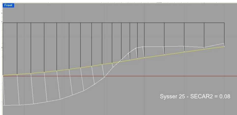
Fig. 5. Stern of the vessel, side view, curvature SECAR 2 = 0.08
