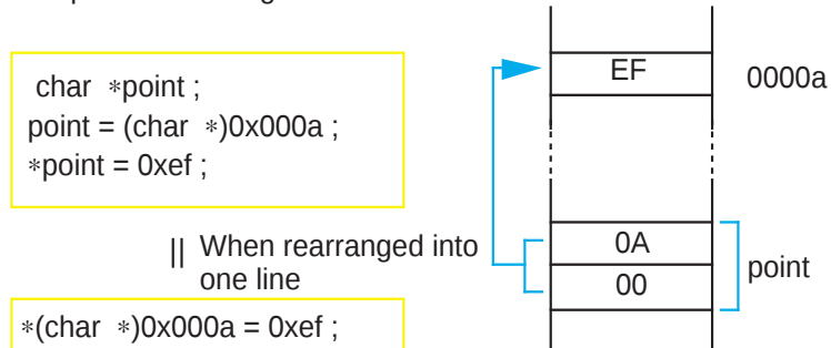
Figure 2.3.8 Specifying absolute addresses using a pointer
