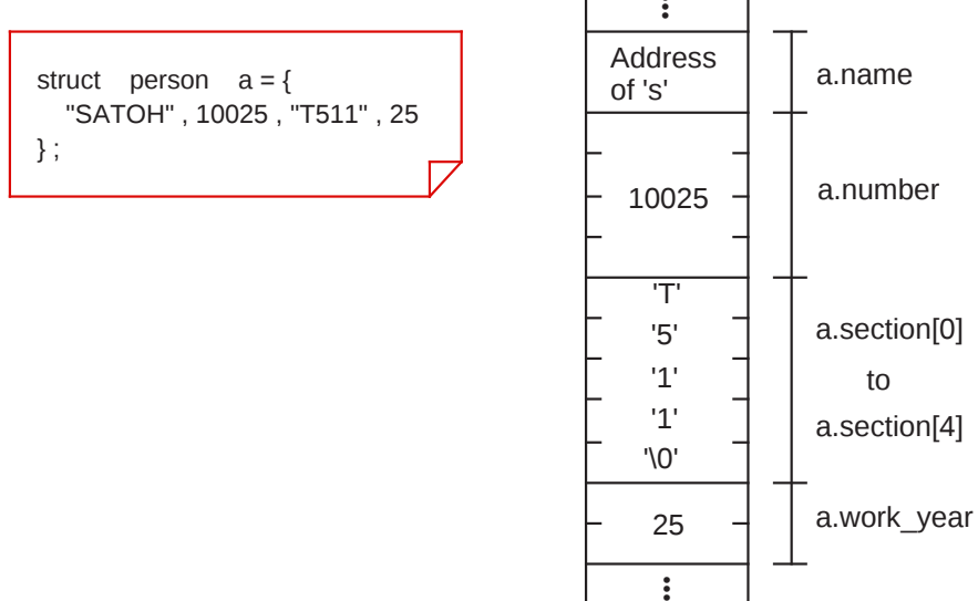
Figure 1.8.2 Struct declaration and memory mapping
