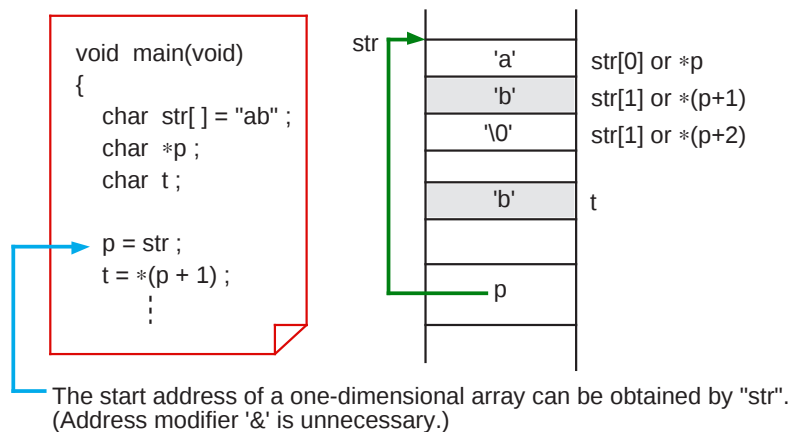
Figure 1.7.6 Pointer variables and one-dimensional array
