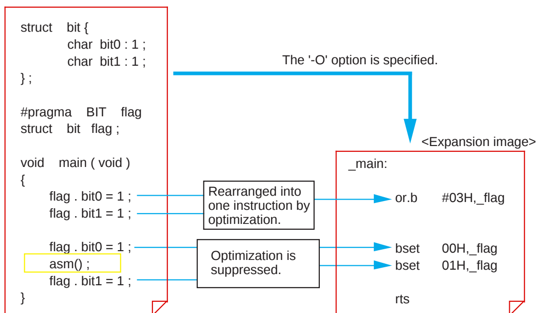
Figure 2.3.13 Suppressing optimization partially by using asm function
