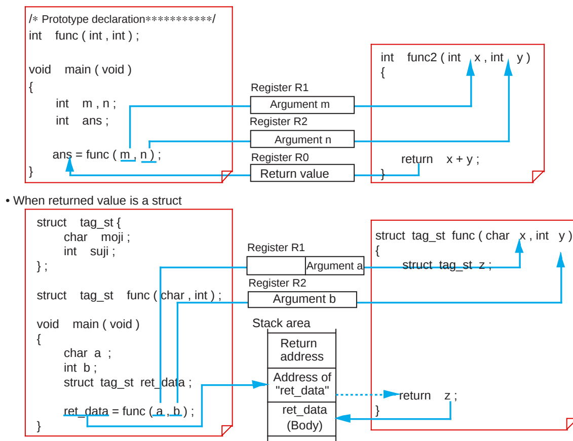
Figure 2.4.5 Example for passing return value
