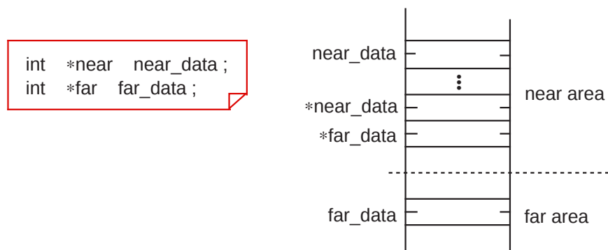
Figure 2.3.4 Specifying area to locate the pointer
