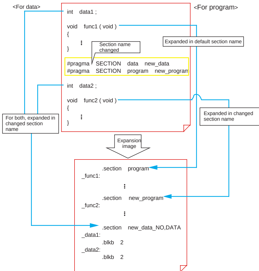
Figure 2.1.5 Typical description of "#pragma SECTION"
