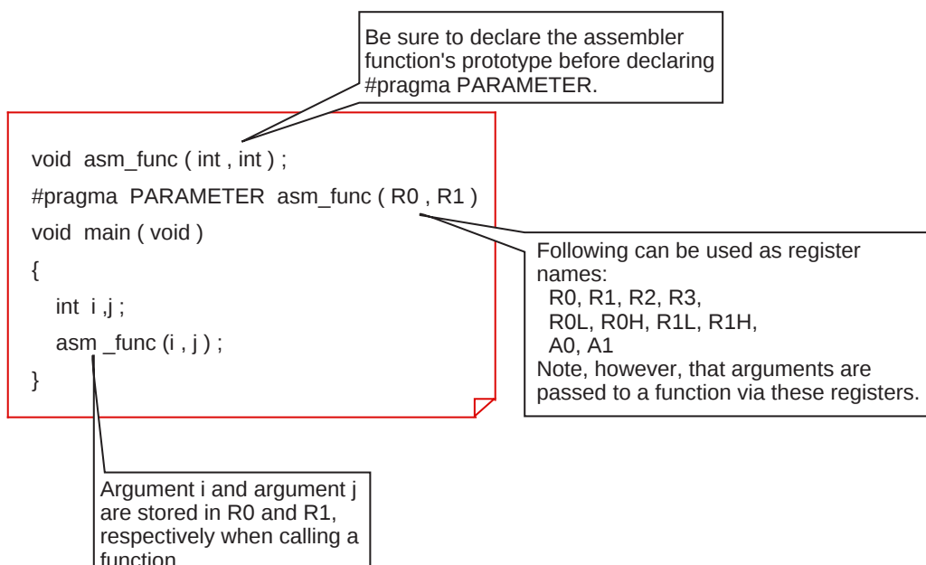
Figure 2.4.7 Example for writing #pragma PARAMETER
