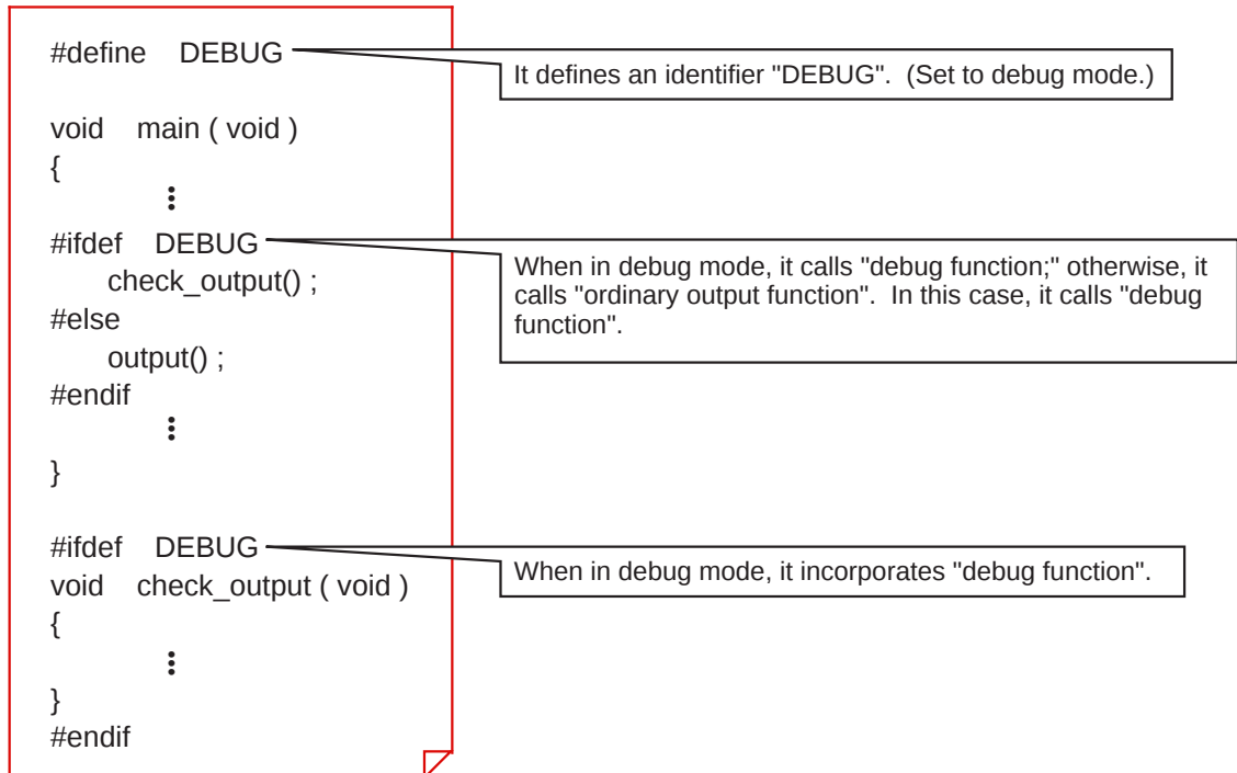
Figure 1.9.5 Example for conditional compile description
