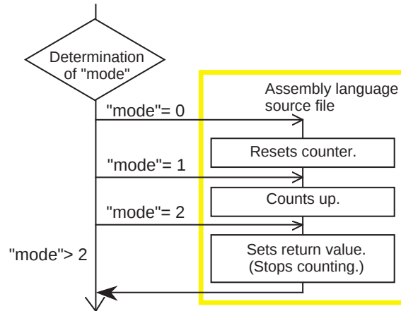
&lt;Assembly language source file&gt;
