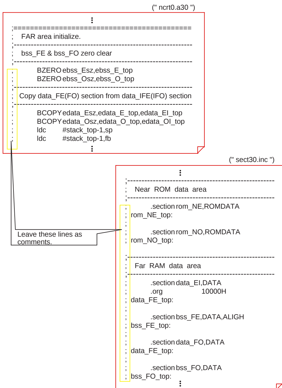
Figure 2.2.13 Example for writing program when operating in single-chip mode
