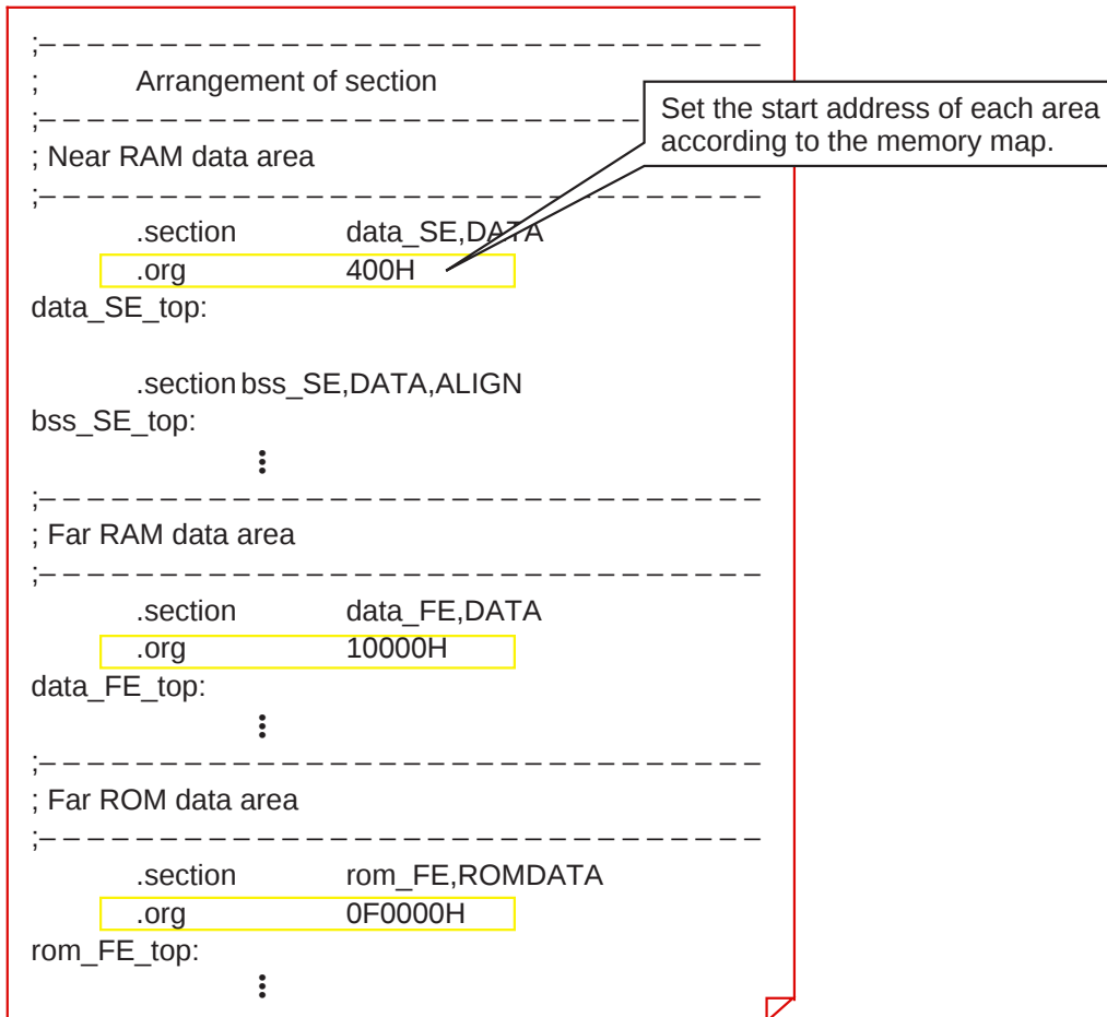
Figure 3.3.5 Modifying memory map
