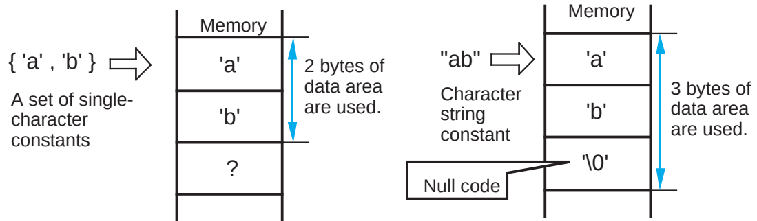
Figure 1.2.2 Difference between {'a', 'b'} and "ab"
