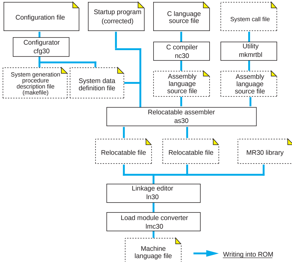
Figure 3.3.7 Development flow
