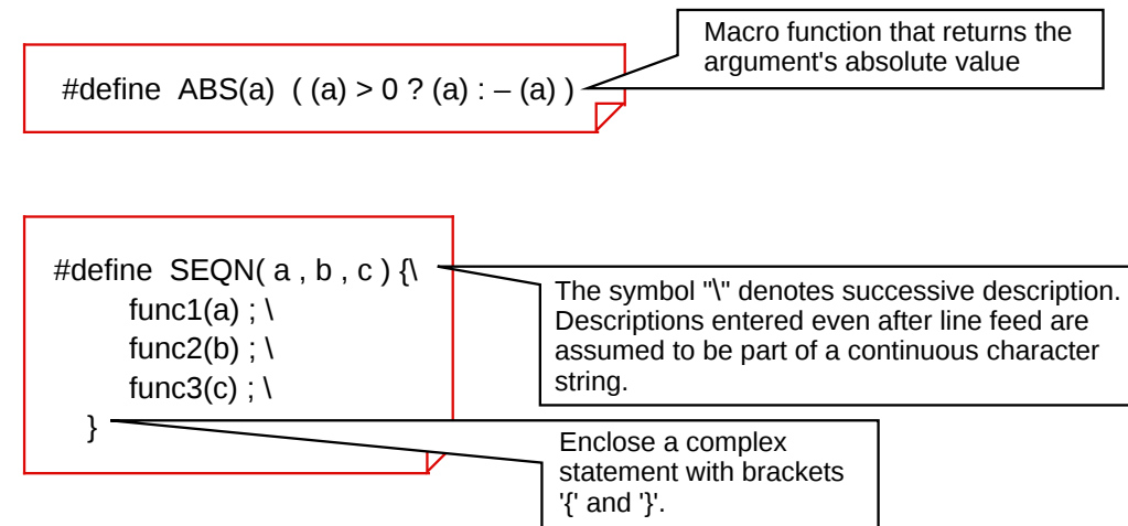
Figure 1.9.4 Example for defining a macro function
