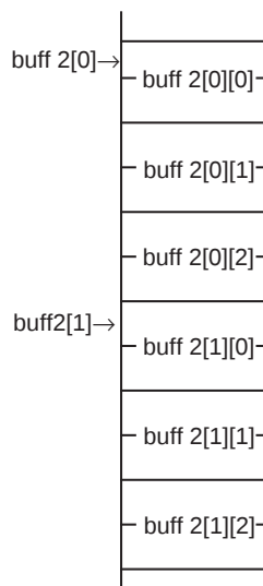
Figure 1.7.3 Declaration of two-dimensional array and memory mapping
