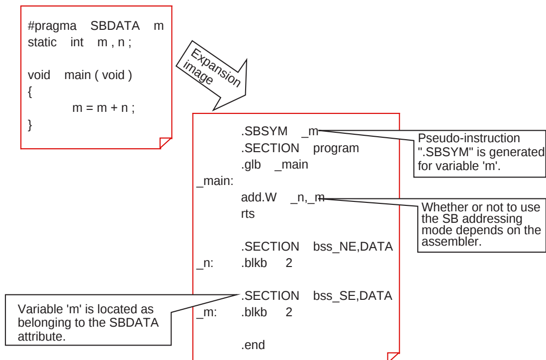
Figure 2.3.5 An image depicting expansion of "#pragma SBDATA"
