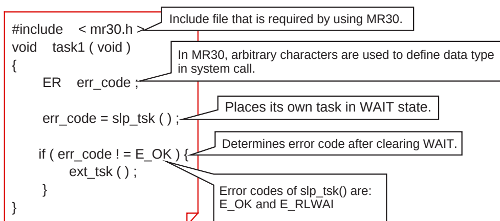
Figure 3.2.4 Utilization of error code
