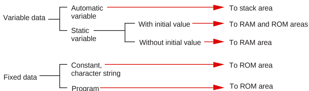
Figure 2.1.1 Types of data and code generated by NC30 and their mapped areas
