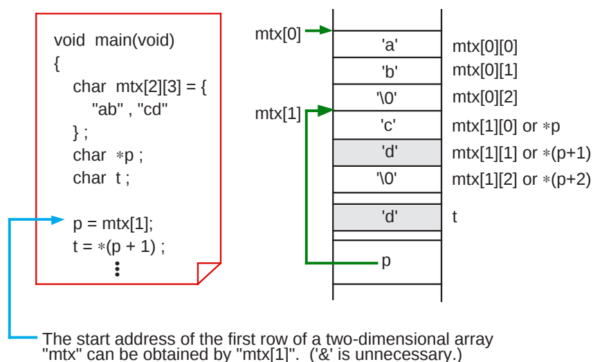
Figure 1.7.7 Pointer variables and two-dimensional array
