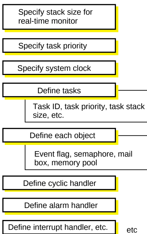
Figure 3.3.6 Outline of configuration file
