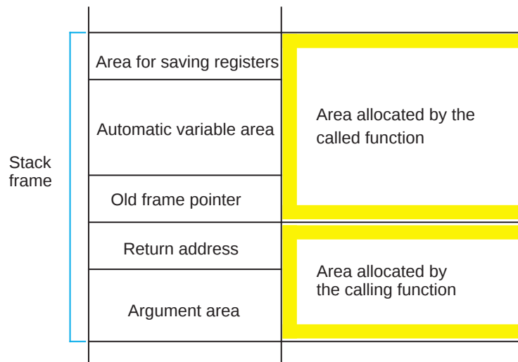
Figure 2.4.2 Structure of a stack frame
