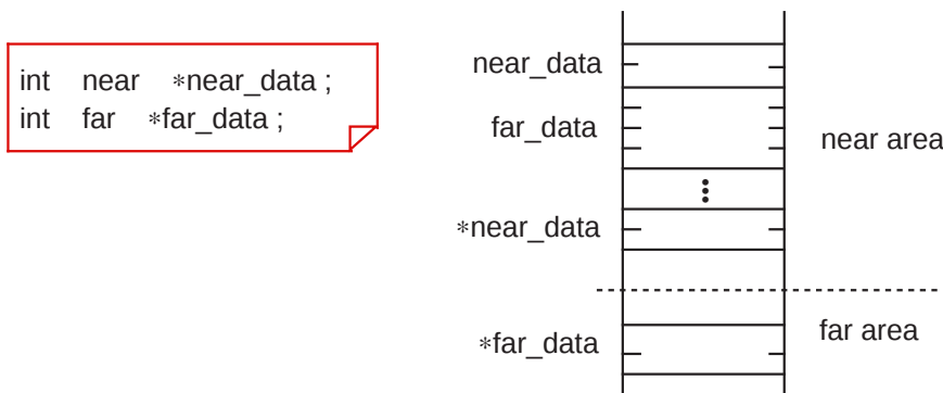
Figure 2.3.3 Specifying address size stored in pointer
