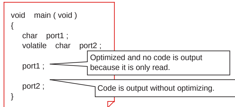
Figure 1.2.6 Example for writing the type qualifier "volatile"
