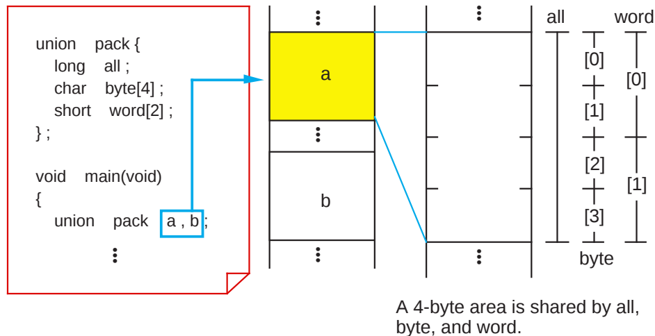
Figure 1.8.4 Declaring and referencing a union
