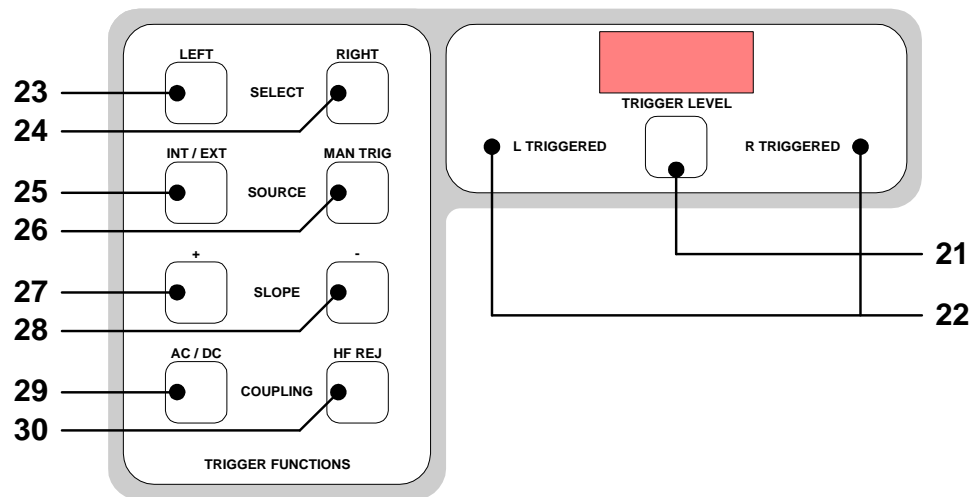
FIGURE 2-3: FRONT-PANEL TRIGGER CONTROLS
