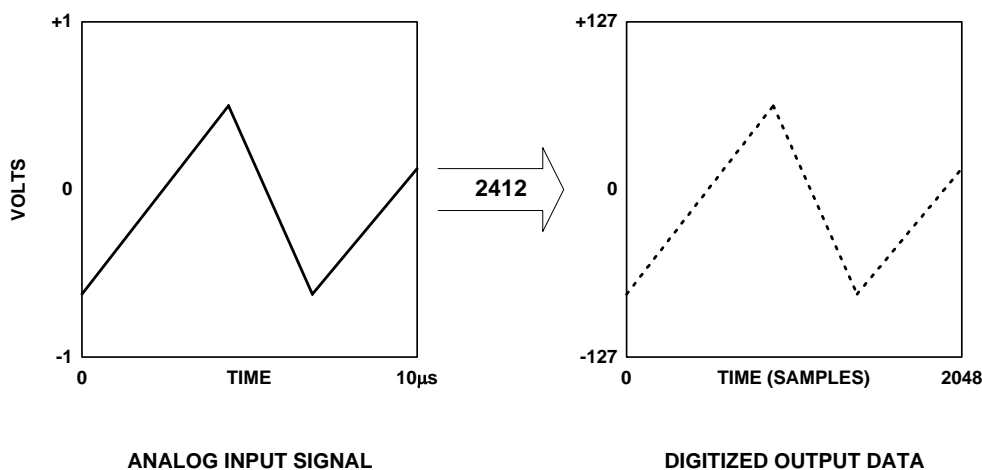
FIGURE 2-14: ANALOG SIGNAL INPUT W/ DIGITIZED DATA OUTPUT
