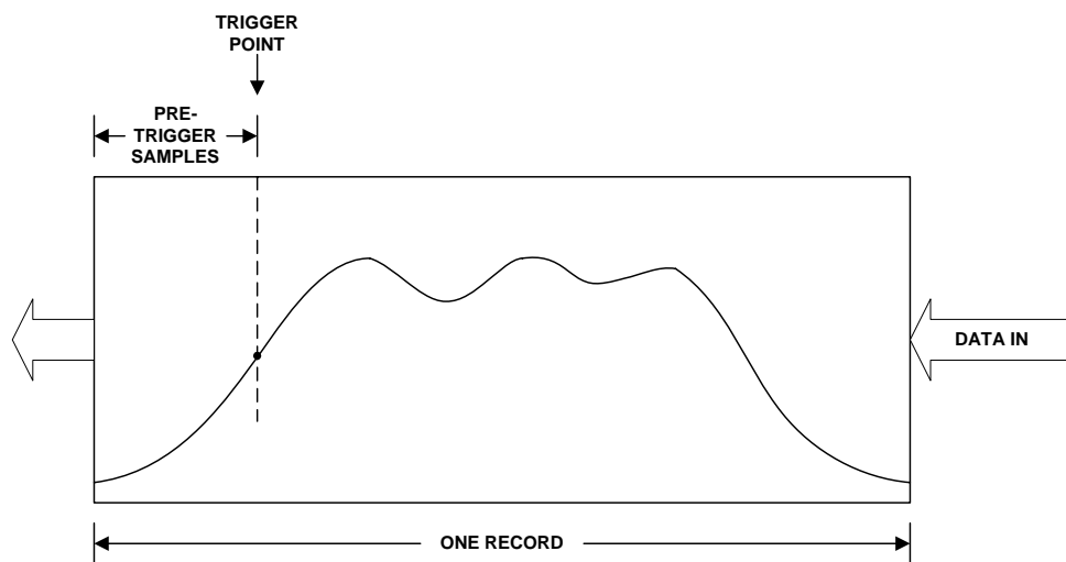
FIGURE 2-10: PRE-TRIGGER ILLUSTRATION
