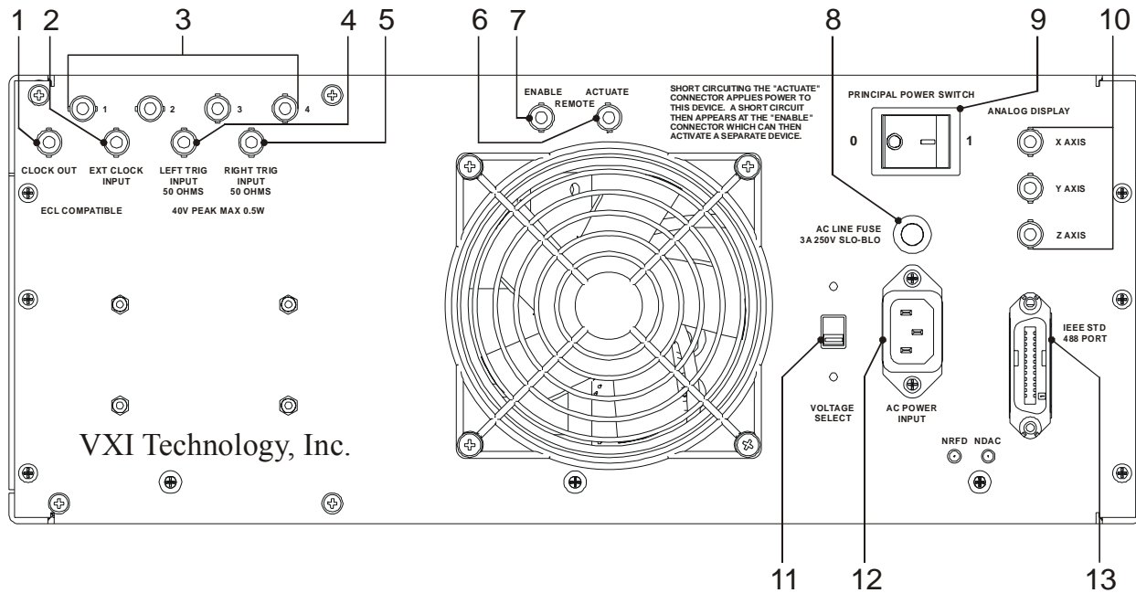
FIGURE 2-5: REAR PANEL CONNECTORS
