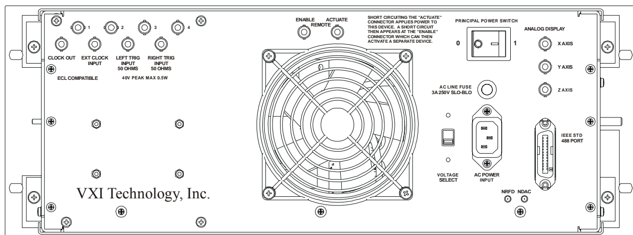
FIGURE 1-2: VT2412-S-11364 DUAL-CHANNEL PROGRAMMABLE DIGITIZER - REAR VIEW
