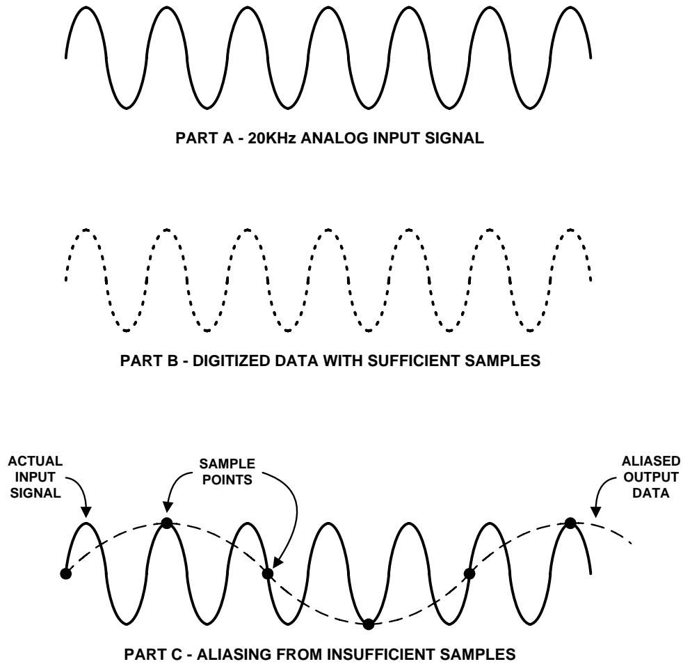
FIGURE 2-16: ALIASING EXAMPLE
