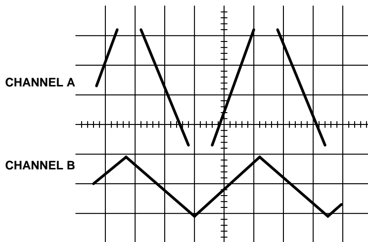
FIGURE 2-17: OUTPUT DATA CLIPPING
