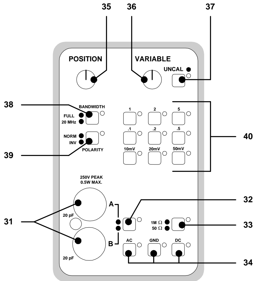
FIGURE 2-4: FRONT-PANEL AMPLIFIER CONTROLS
