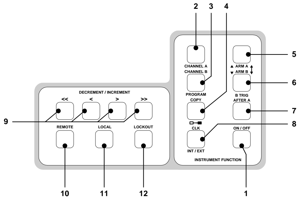
FIGURE 2-1: FRONT-PANEL INSTRUMENT CONTROLS
