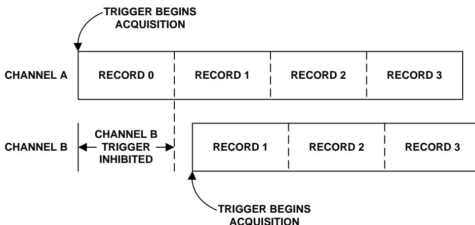
FIGURE 2-13: TRIGGERABLE AFTER A - ILLUSTRATION
