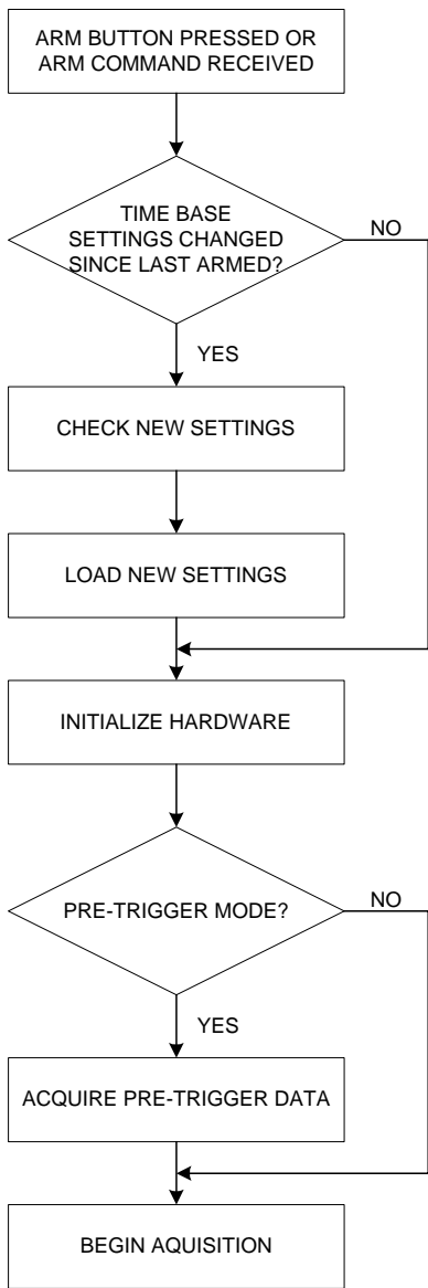
FIGURE 2-6: ARM PROCESS FLOW CHART
