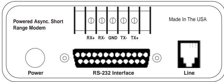
Figure 2. Rear view of 1060 showing interface connectors
