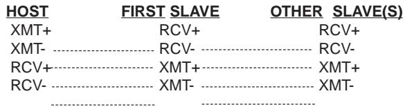
Figure 3. Model 1060 daisy chain wiring
