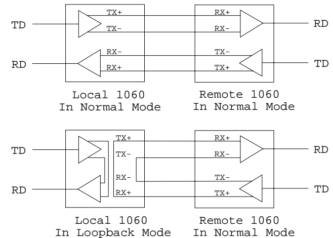
Figure 5. Loopback Test Modes
