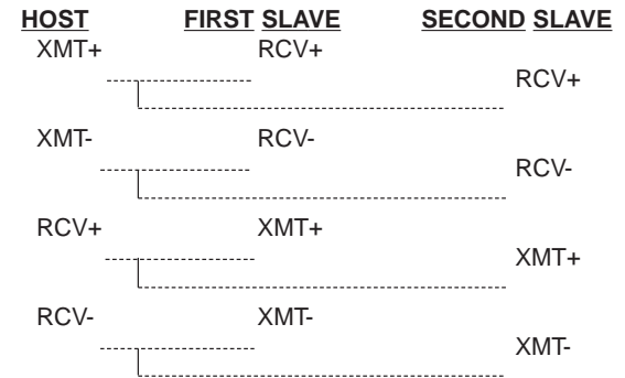
Figure 4. Model 1060 star wiring
