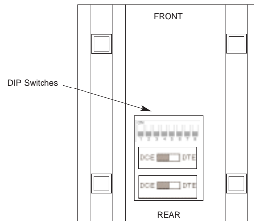
Figure 1. Switch locations underneath Model 1060
