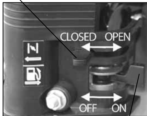
Fuel lever
