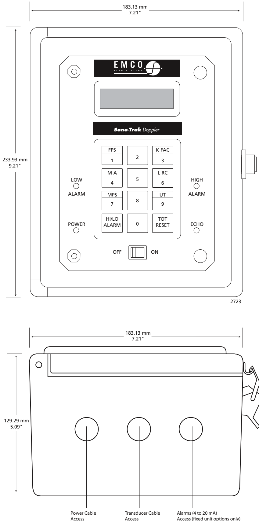
Figure 4-1 Dimensions
