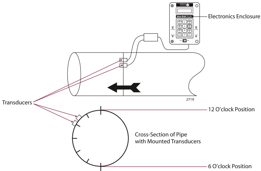
Figure 1 Mount the transducers side by side between 7 and 11 o'clock
