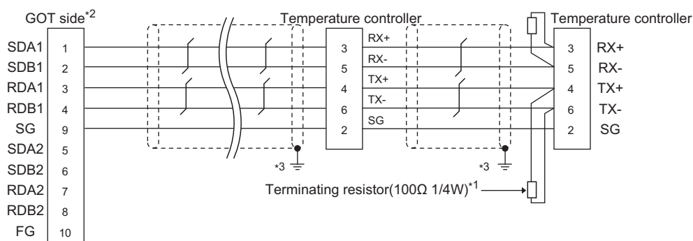
(14) RS-485 connection diagram 14)
