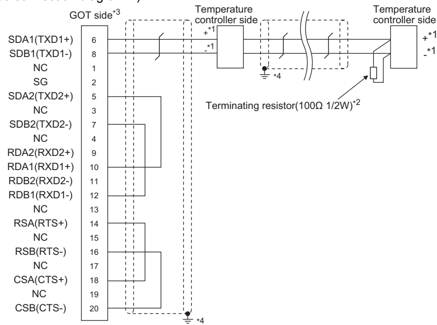
(4) RS-485 connection diagram 4)
