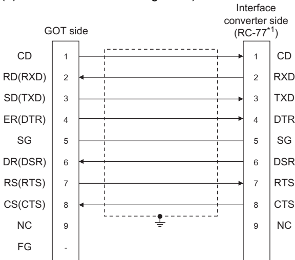
(1) RS-232 connection diagram 1)
