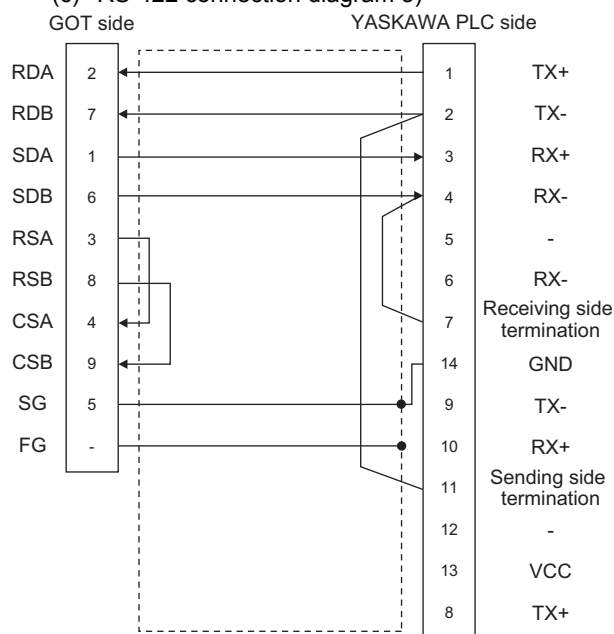
(c) RS-422 connection diagram 3)
