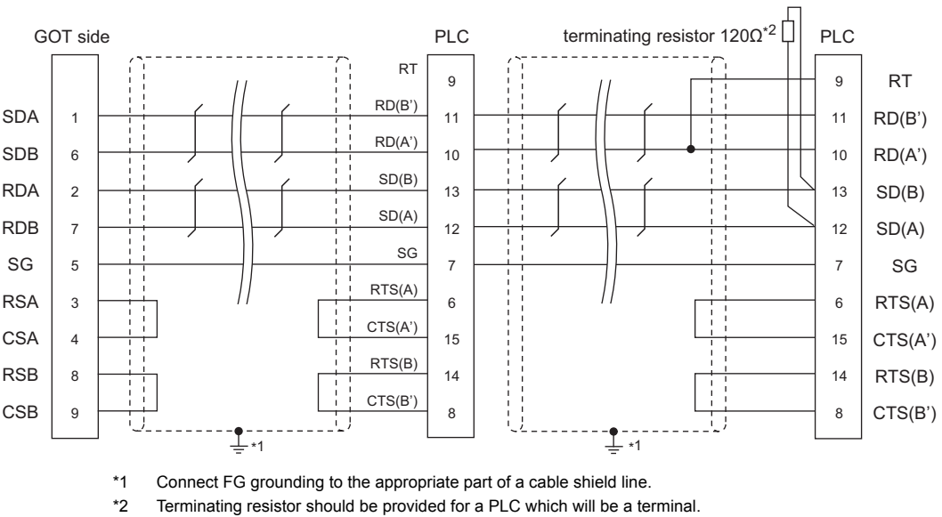
(2) RS-422 connection diagram 2)
