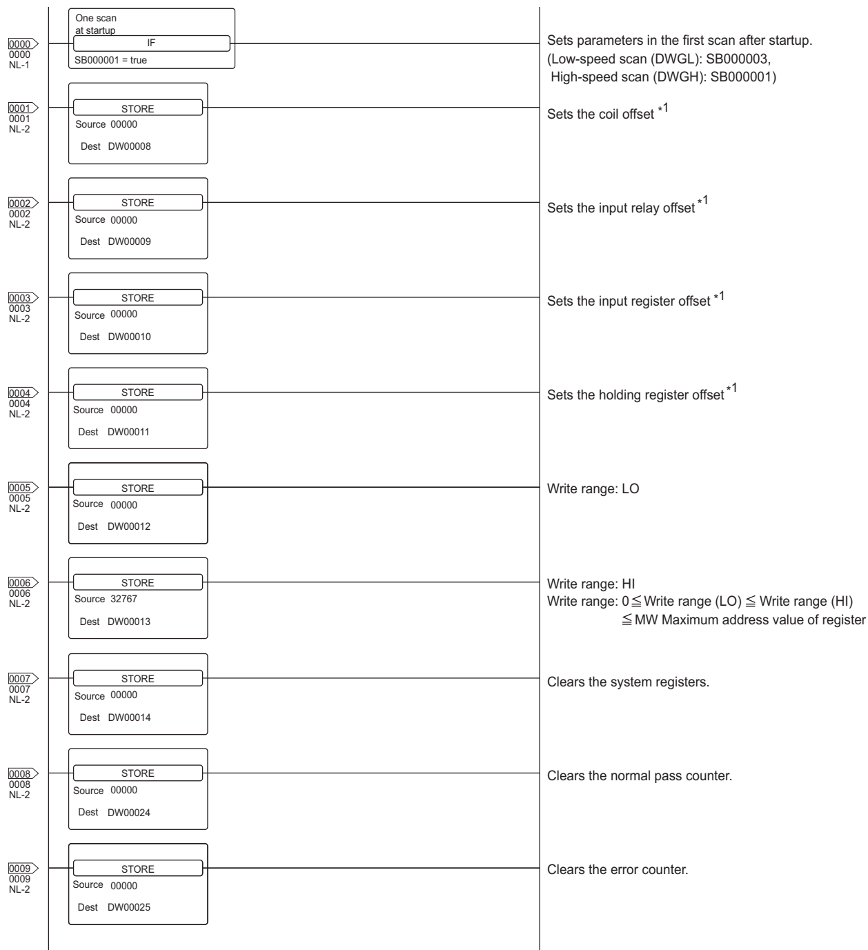
ladder program to receive messages
