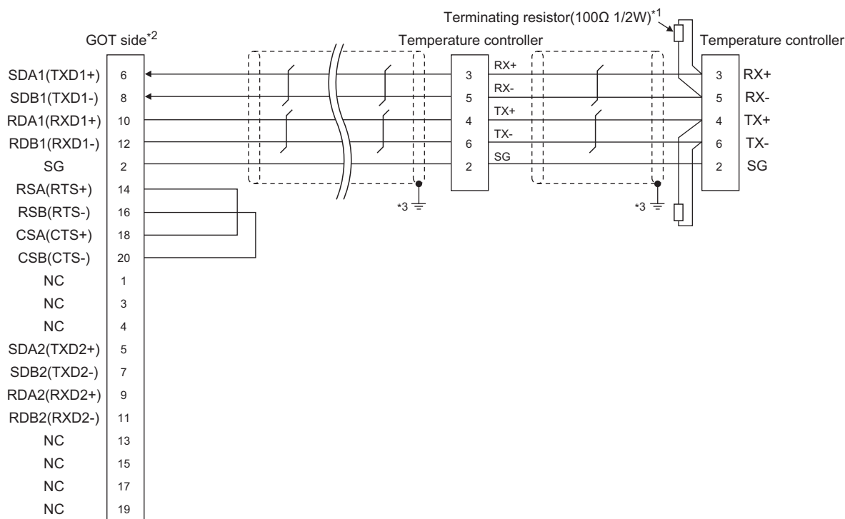
(11) RS-485 connection diagram 11)
