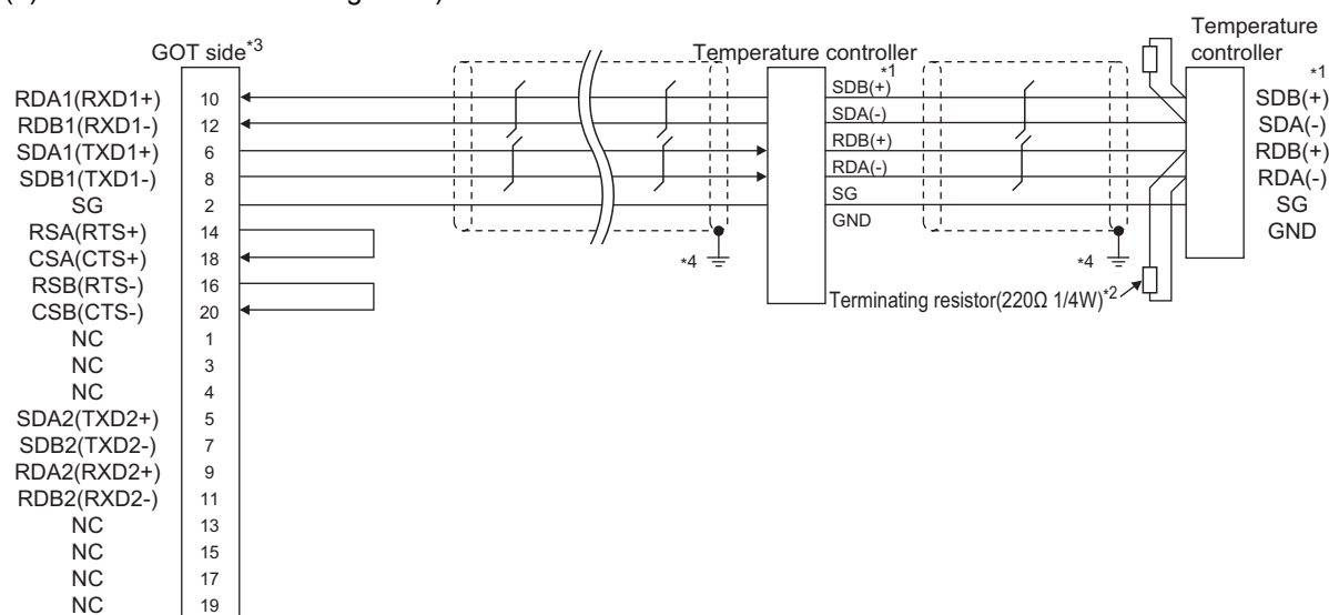
(2) RS-485 connection diagram 2)
