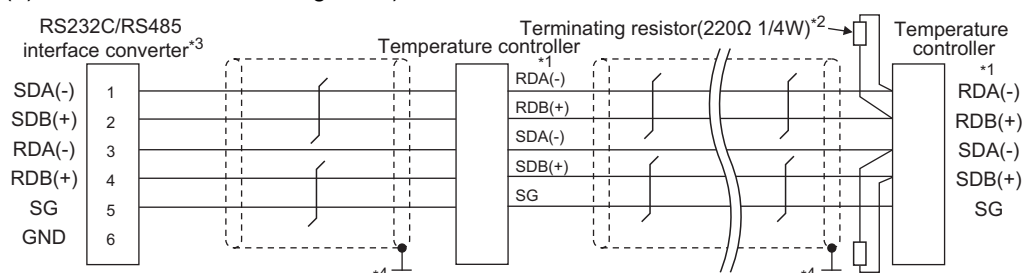
(1) RS-485 connection diagram 1)
