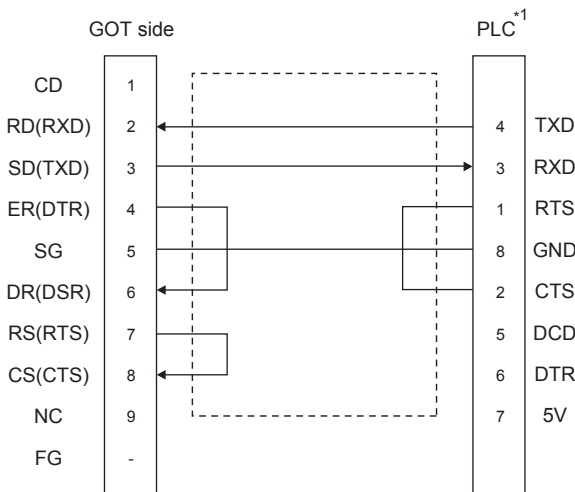
(2) RS-232 connection diagram 2)
