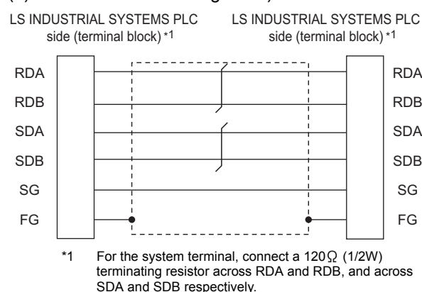
(2) RS422 connection diagram 3)
