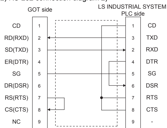
(2) RS-232 connection diagram 2)
