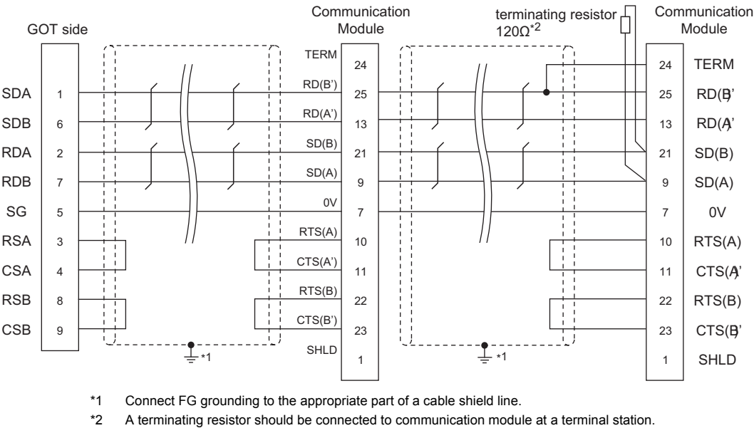
(1) RS-422 connection diagram 1)
