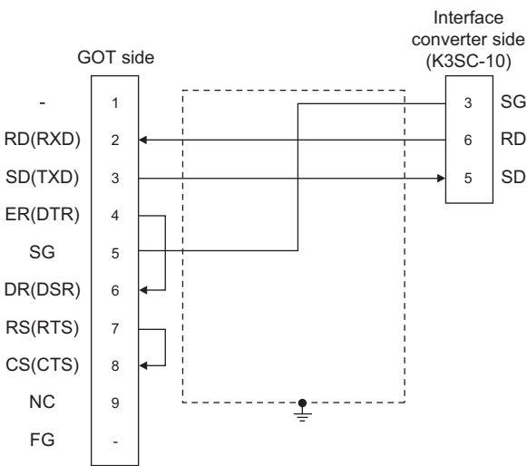
(3) RS-232 connection diagram 3)
