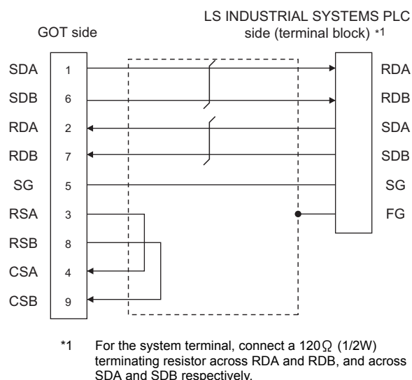
(2) RS422 connection diagram 3)
