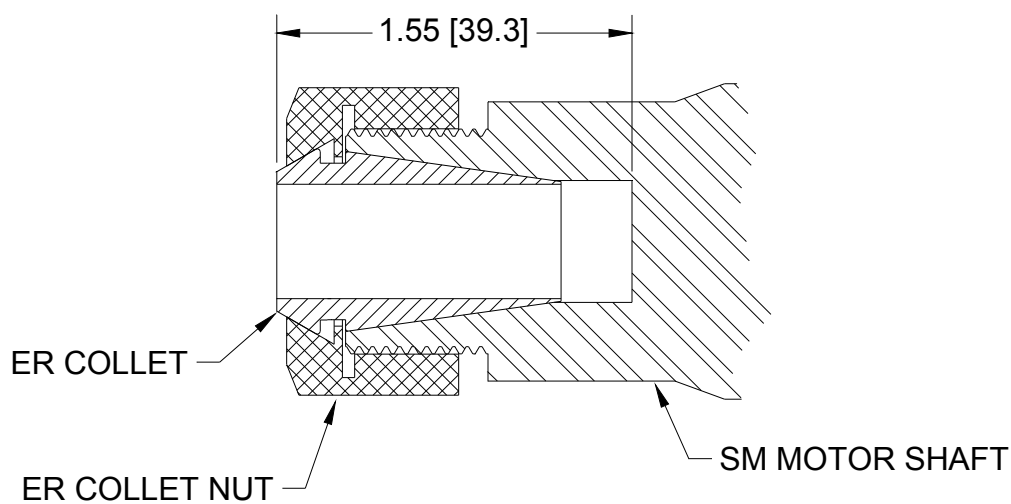
Figure 6. SM0605 Collet Drawing
