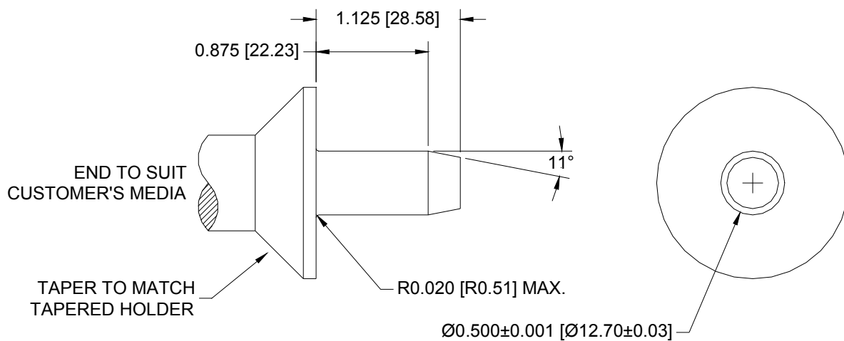
Figure 7. STC0605 & SM0605 Toolholder Drawing
