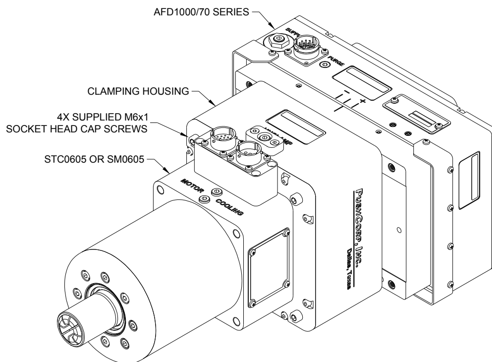
Figure 2. 0605 Perpendicular-Axis Configuration
