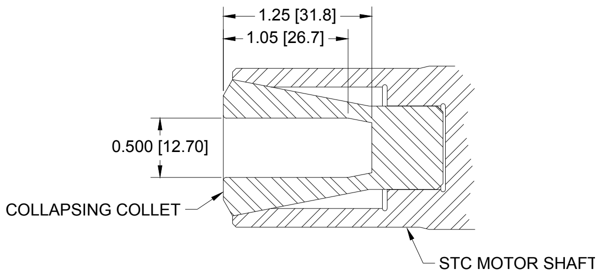
Figure 5. STC0605 Collet Drawing
