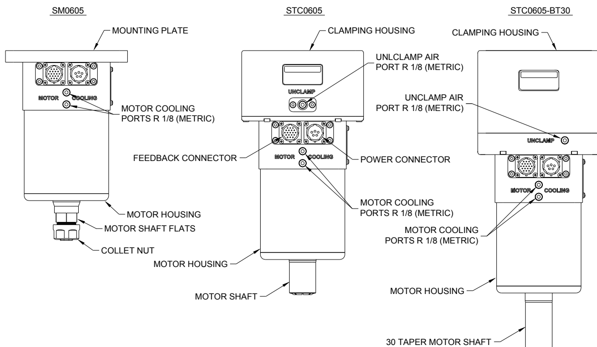
Figure 13. 0605 External Features
