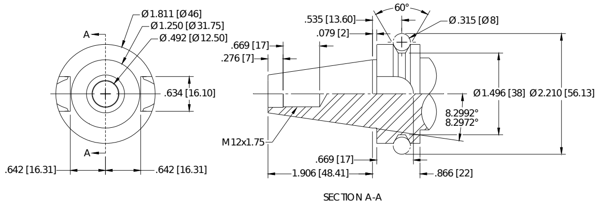
Figure 8. BT30 Toolholder Dimensions
