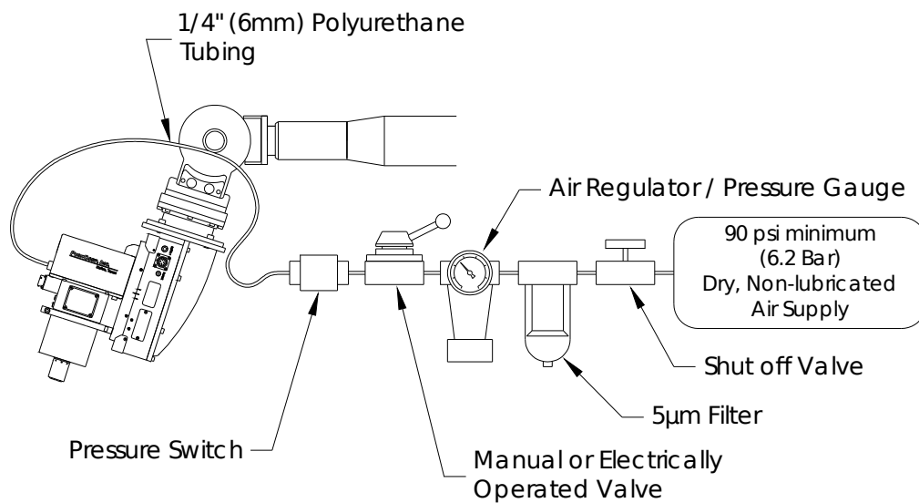
Figure 11. Pneumatic Connections
