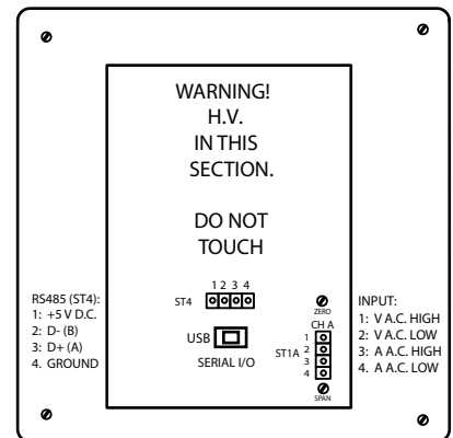
NTM-M & -N TYPICAL CONNECTIONS SIGNAL POWER MODELS
