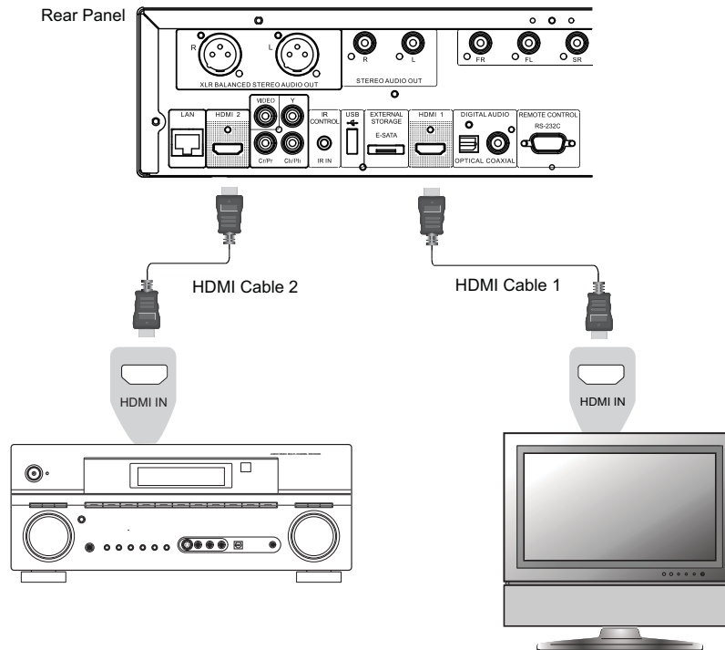
Method 10 – Dual HDMI Connection
