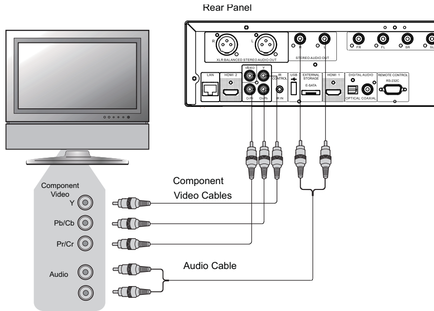
Method 4 – Component Video Connection to TV
