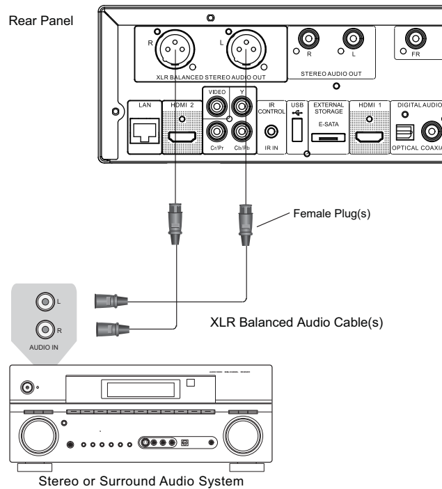
Method 9 – Stereo Analog Audio Connection by Balanced cables
