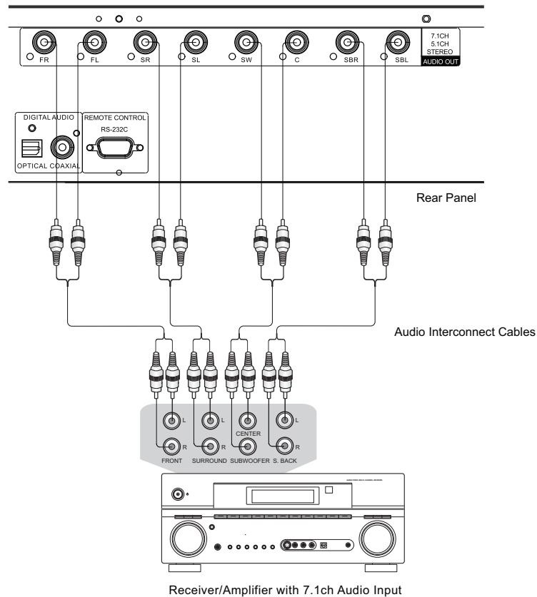
Method 6 – 7.1ch Analog Audio Connection
