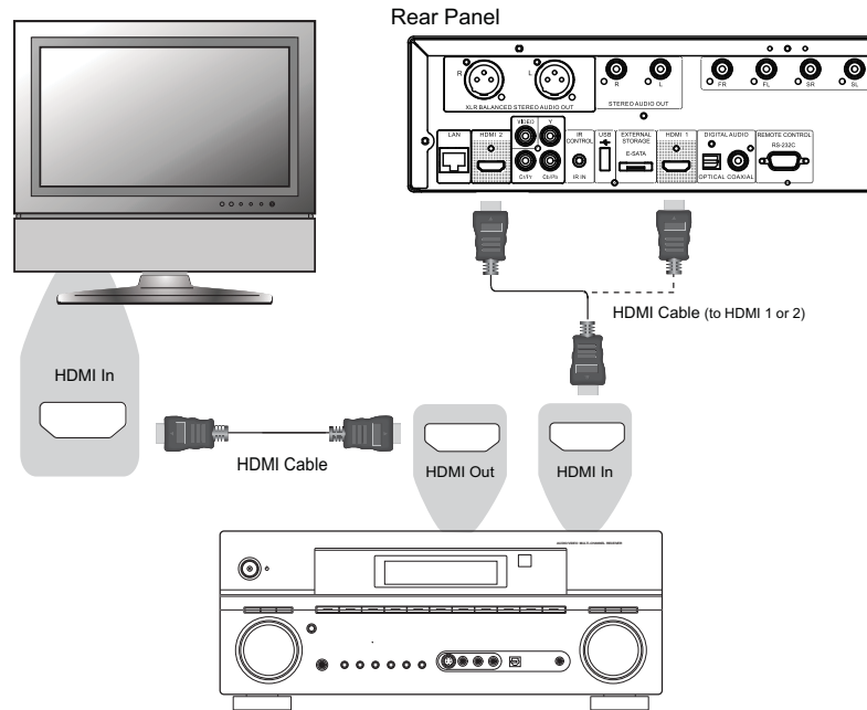
Method 5 – HDMI Connection to Receiver and TV
