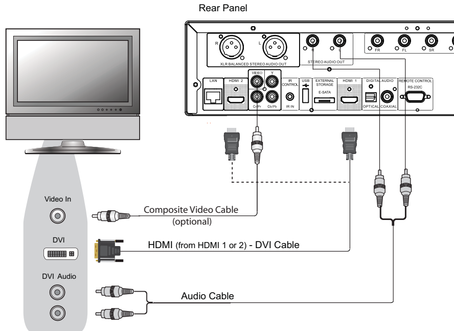
Method 3 – DVI Connection to TV
