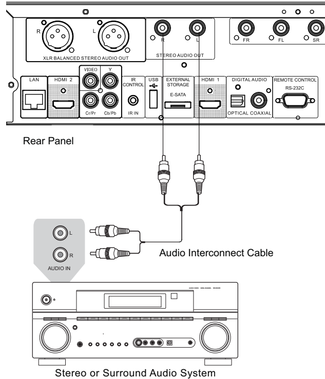
Method 8 – Stereo Analog Audio Connection by RCA cables
