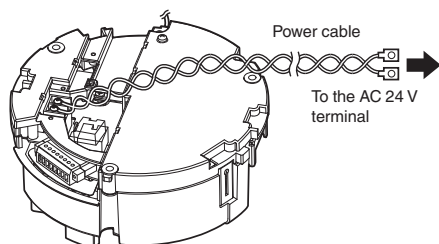
Power cord for connecting to AC 24 V (Reference value)
