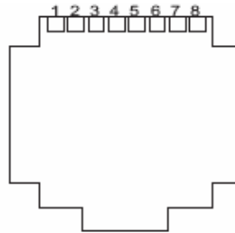
Fig. 5-4 RJ-45 Connector.
