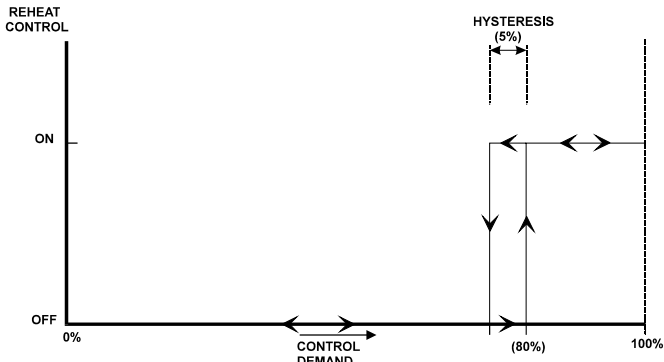
Fig. 11. Reheat switching and hysteresis (defaults shown)
