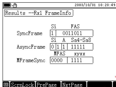
Figure 6.11 Frame Information
