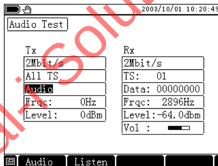
Figure 6.6 Audio Test Result
