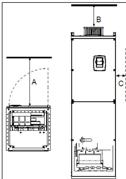
Fig. 7. NXS FR10 – FR11 (NXS0385... - NXS0730...) installation space
