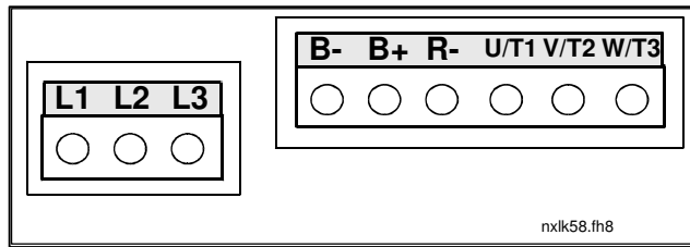
Fig. 8. NXS power connections FR4-FR6 in FR7-FR11 connectors B-, B+ and R- do not exist as standard.
