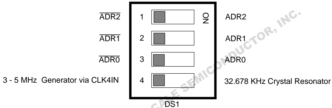
FIGURE 2-2 Configuration Dip-Switch - DS1
