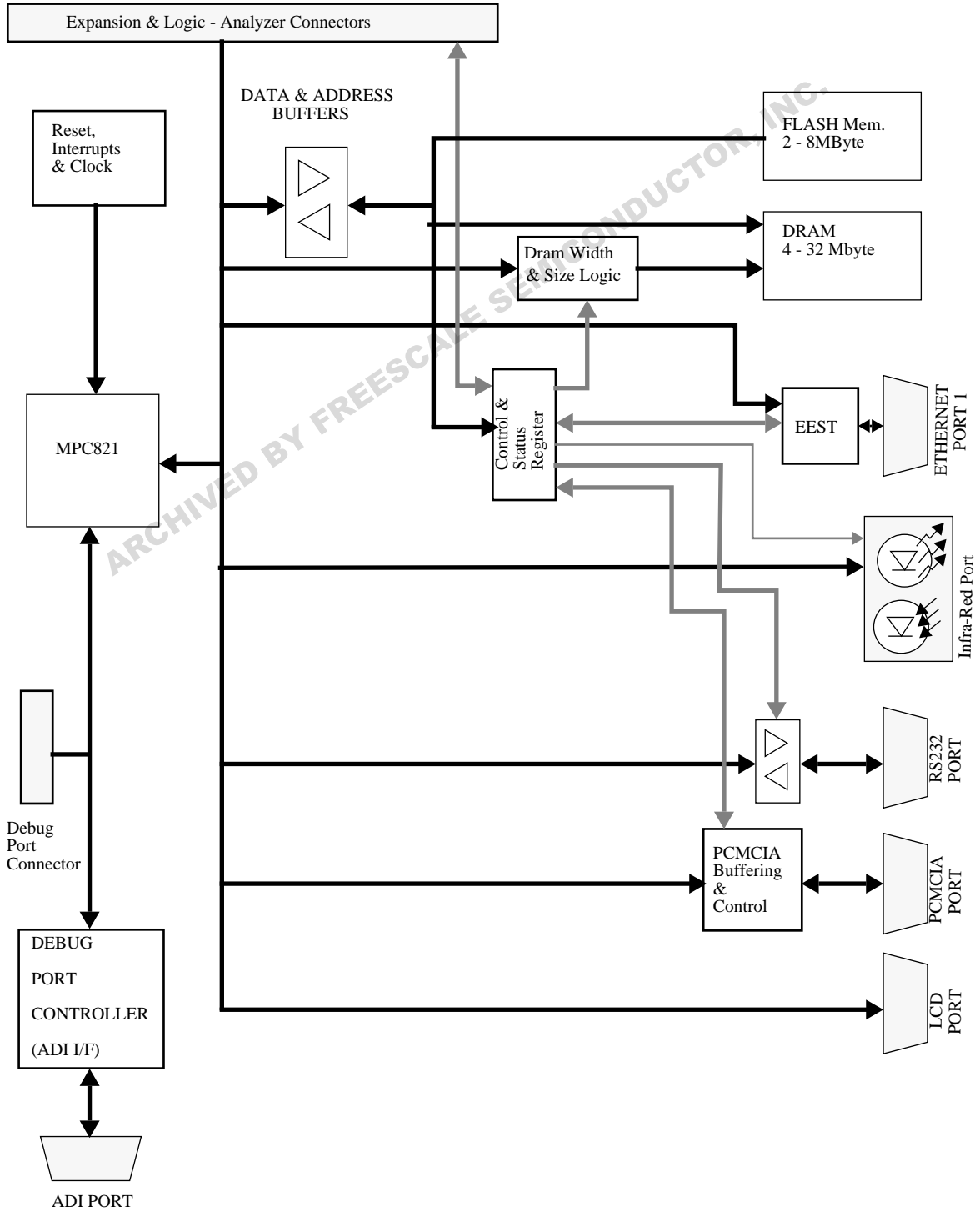
FIGURE 1-1 MPC821ADS Block Diagram
