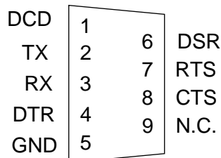
FIGURE 4-4 RS232 Serial Port Connector
