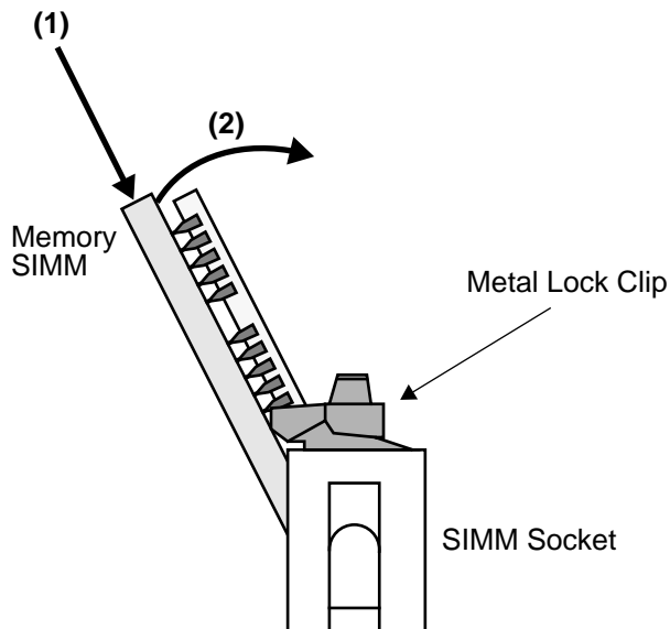
FIGURE 2-14 Memory SIMM Installation
