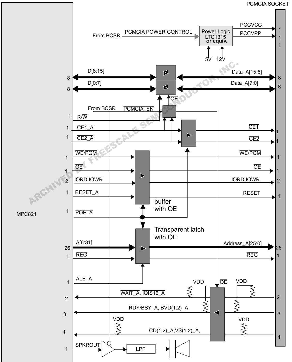
FIGURE 4-5 PCMCIA Port Configuration
