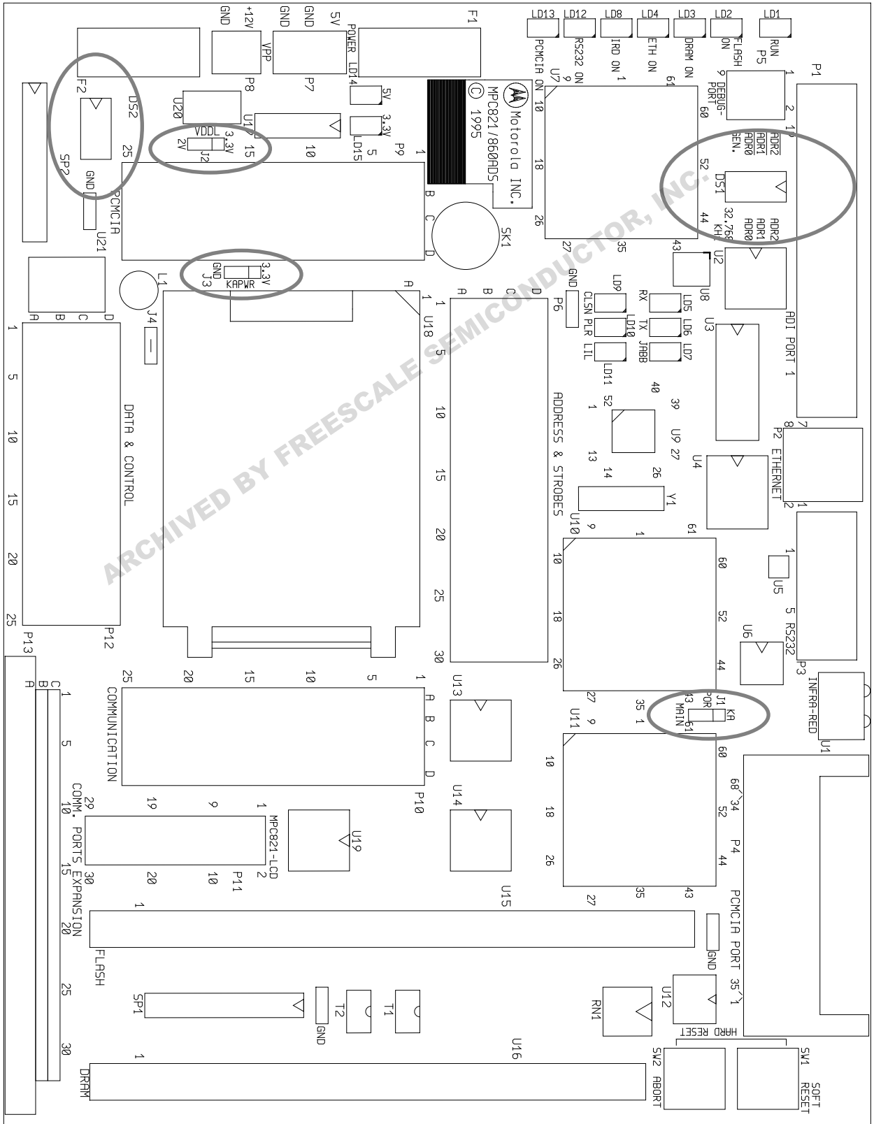
FIGURE 2-1 MPC821ADS Top Side Part Location diagram
