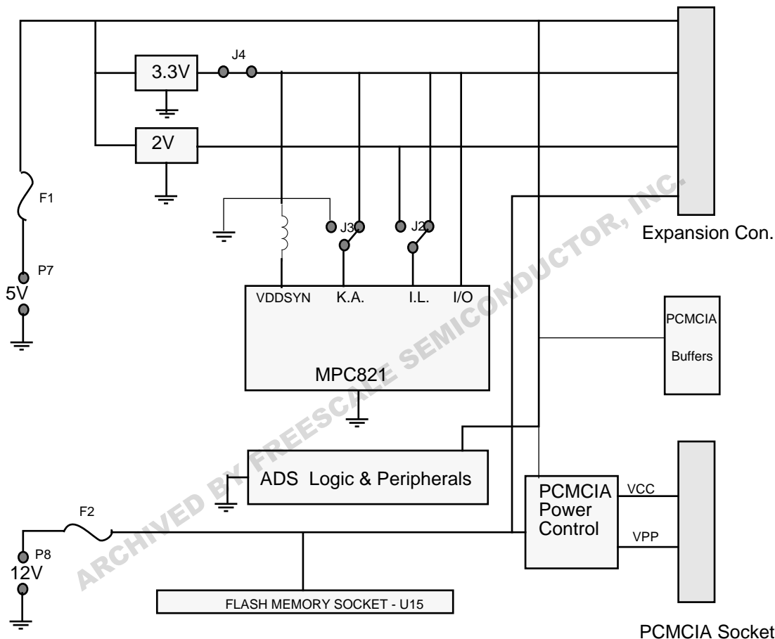
FIGURE 4-8 MPC821ADS Power Scheme
