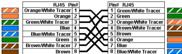
Color Standard EIA/TIA T568B Ethernet Crossover Cable
