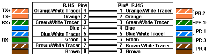
Color Standard EIA/TIA T568B Ethernet Patch Cable
