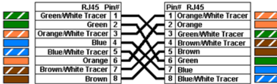
Color Standard EIA/TIA T568A Ethernet Crossover Cable
